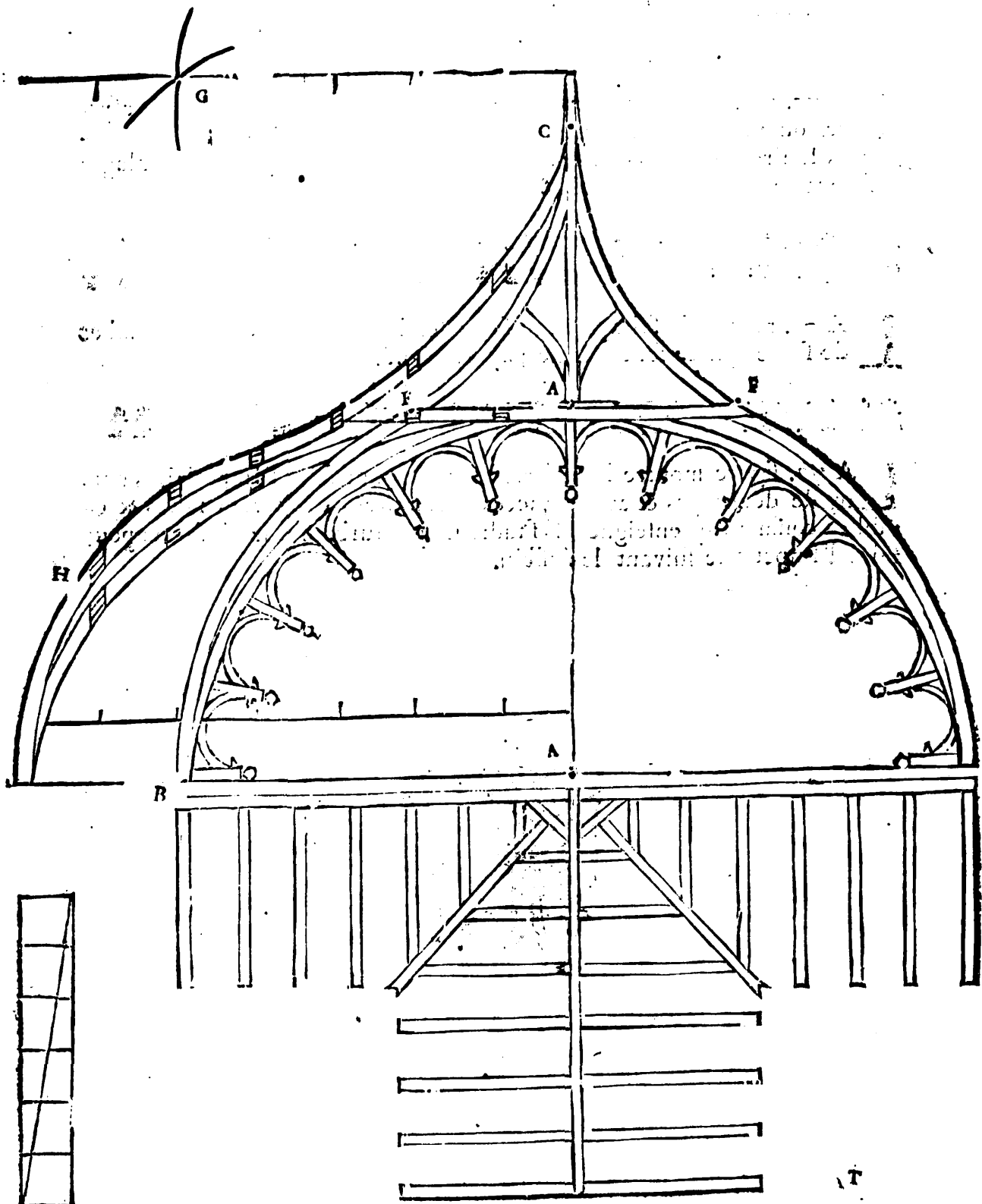
LXXV. LXXVI. FIGURE.
