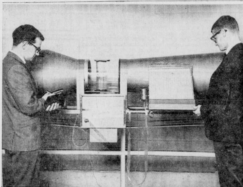
Messrs. Mercier and Boucher are running an experiment on the 12-inch wind tunnel of the Hydraulic Laboratory. The pressure distribution on a symmetrical airfoil is being studied.
