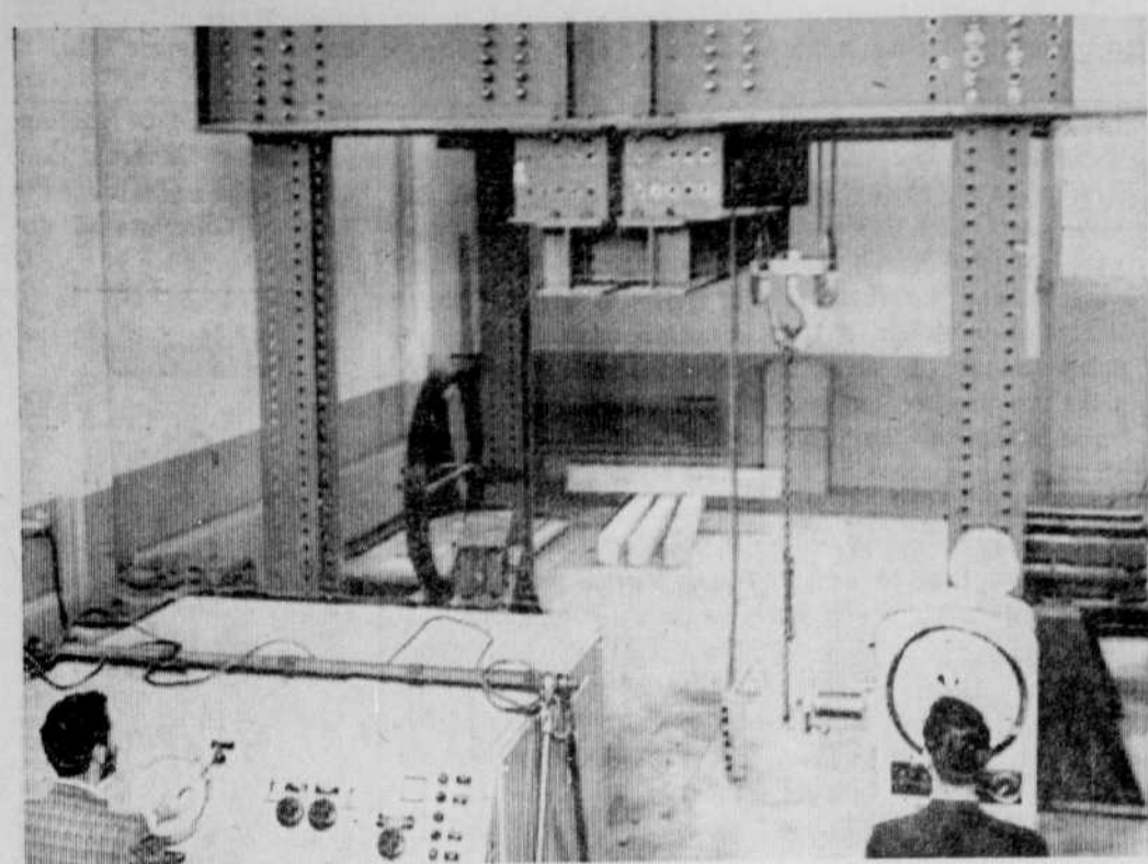
Messrs. Bergeron and Cyr are operating the hydraulic machine on the test bed. This bed is used to test large specimens such as concrete beams, truss or any structural members.
