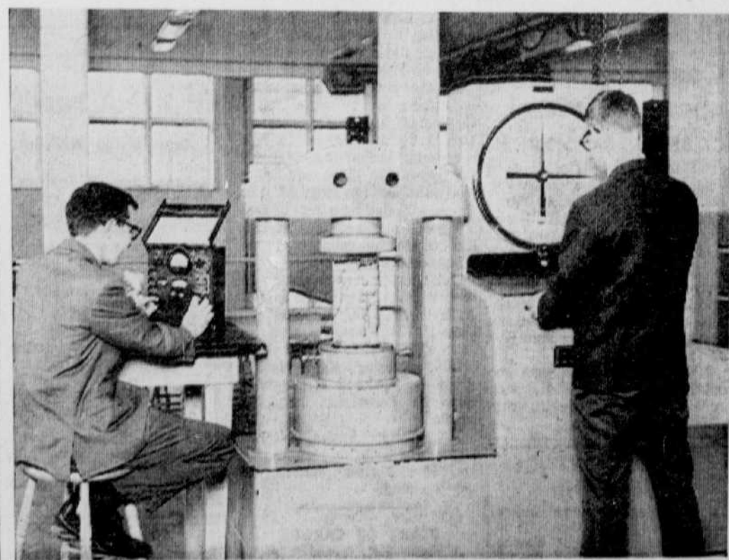
Messrs. Mercier and Boucher are working on a compression test of a concrete cylinder, reading the stress and strength. The machine has a maximum capacity of 300,000 pounds.
