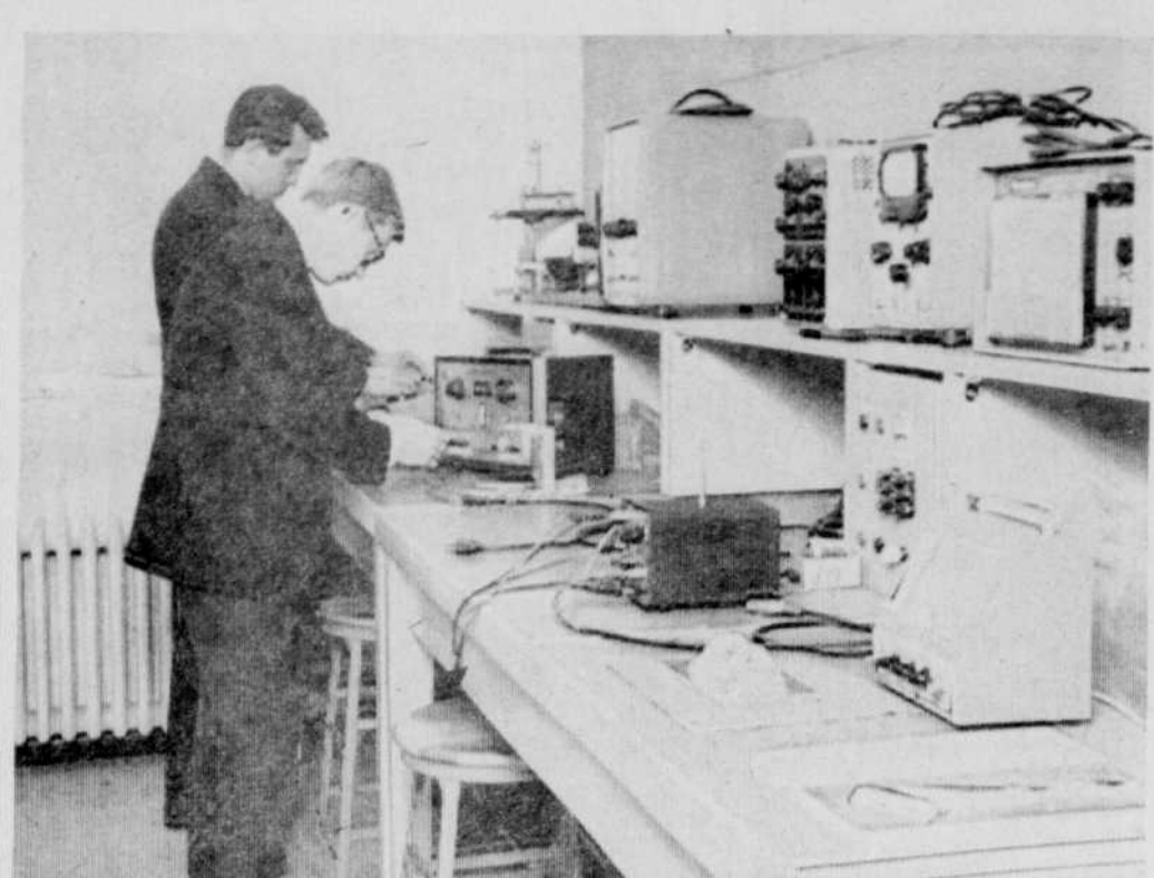
Calibration of electric strain gages in the applied mechanics laboratory. At work: Yvon Mercier and Normand Lessard.
