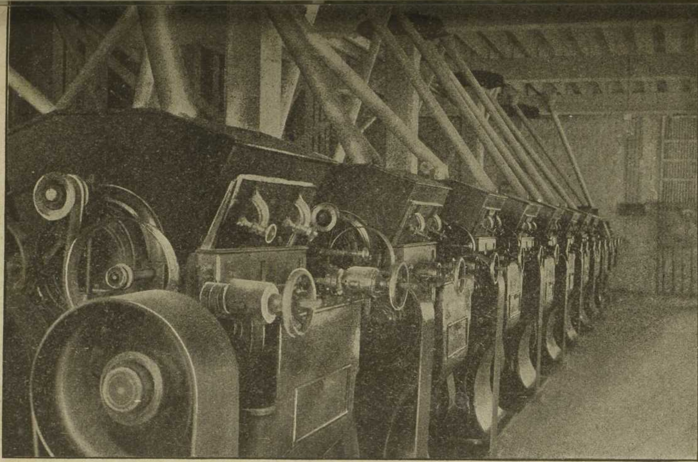
ETAGE DES ROULEAUX, MOULIN ROYAL. THE OGILVIE FLOUR MILLS COMPANY, LIMITED, MONTREAL.
