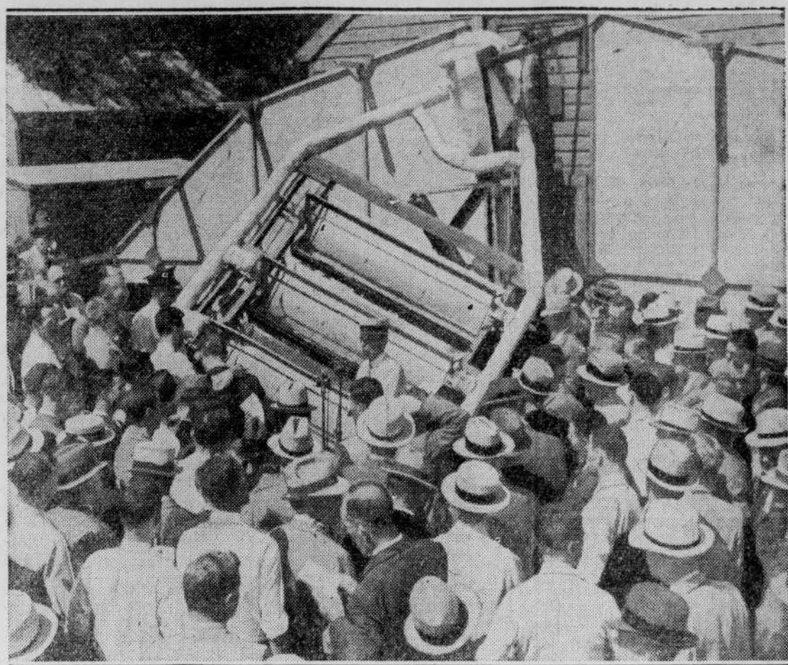
Photo shows Dr. Charles G. Abbot, secretary of the Smithsonian Institution, as he demonstrated his Solar Heat Collector before a large gathering of delegates to the Third World Power Conference in Washington, D.C. The three curved mirrors collect enough solar heat to generate steam sufficient to produce one half horsepower.
