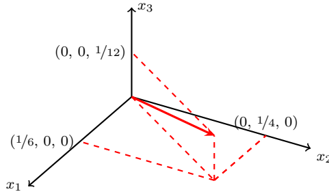
Figure 9: Three-dimensional interior direction (\bar{v}_1^0, \bar{v}_2^0, \bar{v}_3^0) = (1/6, 1/4, 1/12) with P = \emptyset and w = 1
