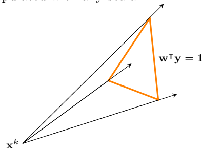
Figure 2: At \mathbf{x}^k , the cone \{y \geq 0 \mid \mathbf{K}\mathbf{y} = \mathbf{0}\} \subseteq \mathbb{R}_+^{2n} cut by \mathbf{w}^\top \mathbf{y} = 1
