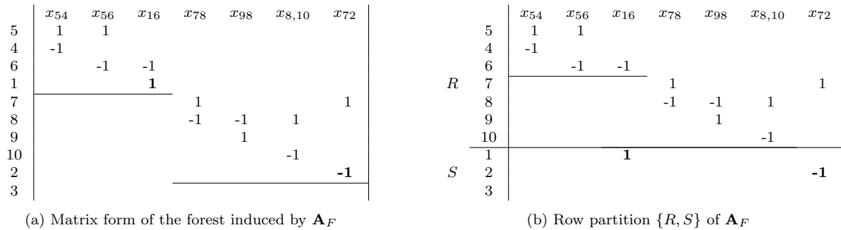
Figure 3: Network flow problem row partition
