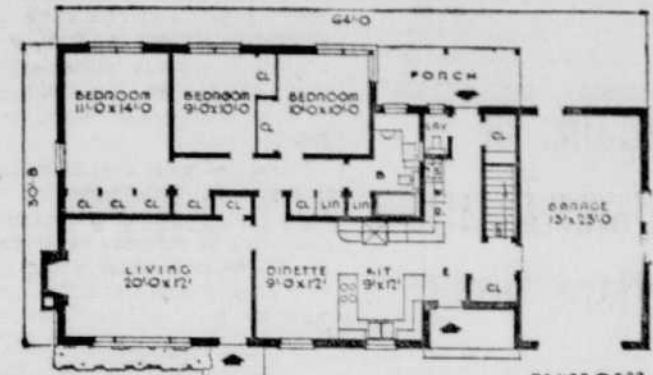
A SMALL HOUSE PLANNING BUREAU DESIGN NO. C-522
