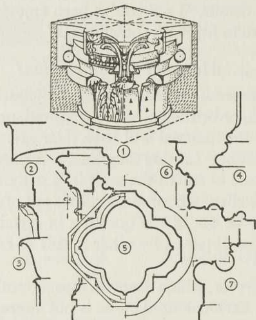
FIG. 158. The effect of banking and jointing on the detail of masonry.
