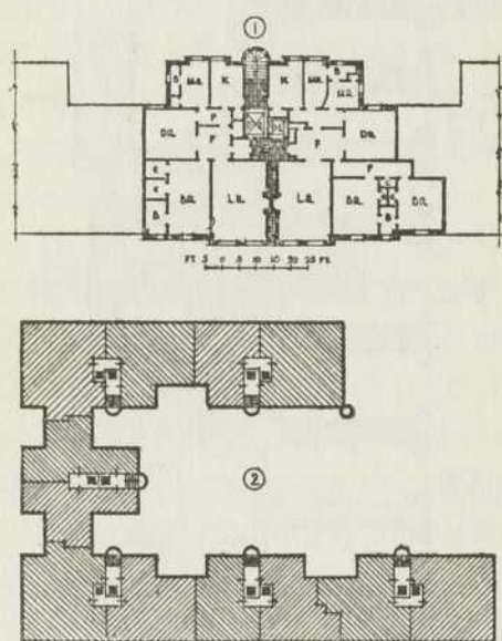
FIG. 132. Chateau Apartments, Montreal (Ross and McDonald).
