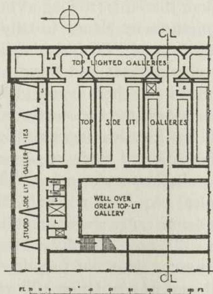
FIG. 127. Part plan for a picture-gallery with varied lighting systems.
