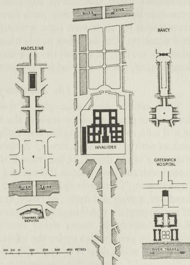
FIG. 133. Some notable plans in the grand manner.
