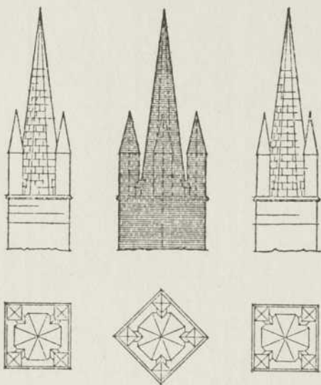
FIG. 61. The correction for corner pinnacles.
