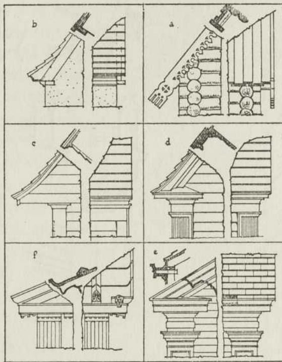
FIG. 159. Verges and Eaves.
