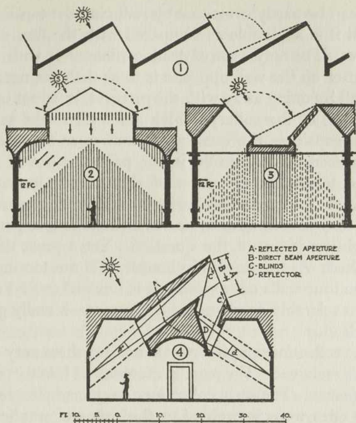
FIG. 126. 1. Sawtooth roof light facing N. 2. Filtered sunlight, Champeau method. 3. Top-side lighting, Seager method. 4. Direct and reflected N. light, Nobbs method.
