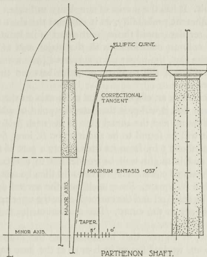
FIG. 75. Setting out for entasis by means of a conoid with tangential correction.
