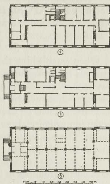
FIG. 134. 1, 2. Upper and main floors of Pulp and Paper Institute, Montreal—space distribution. 3. Main floor plan—distribution of points of support and framing.
