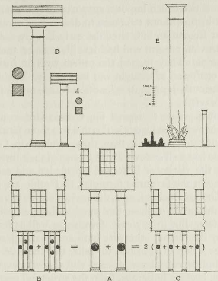
FIG. 46. A, B, C show a constant load carried on orders differing in scale in the ratio 1 : 2.
