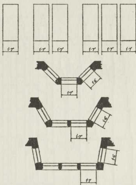
FIG. 58. Corrections for bay window side-lights.
