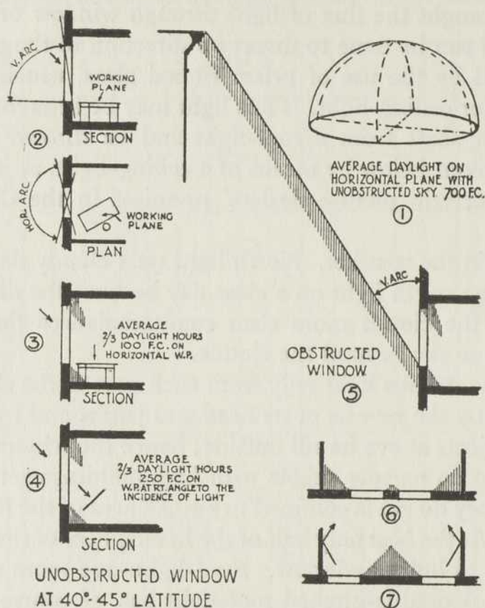
FIG. 123. Light from the sky entering windows. Rough working average.
