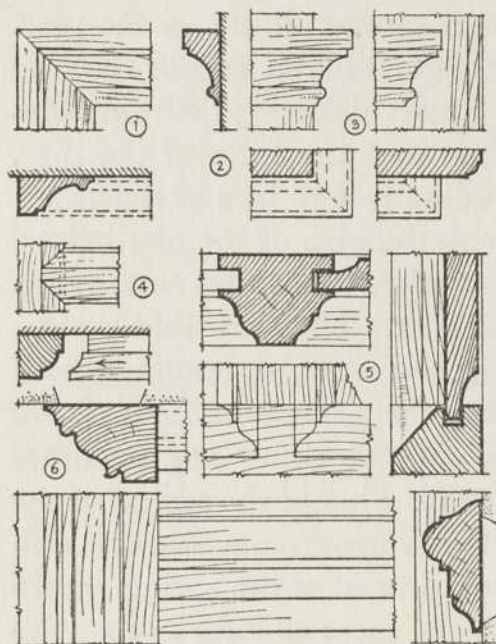
FIG. 164. The disposal of mouldings in joinery.
