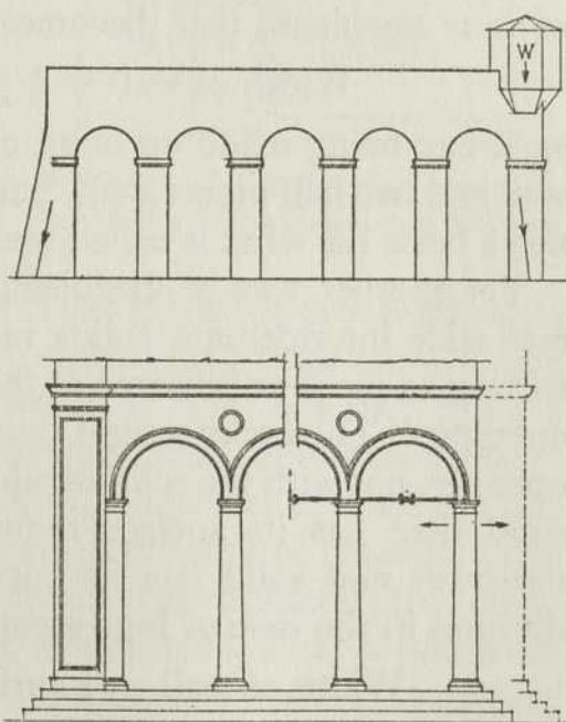
FIG. 146. The strong end solid required in arcades, otherwise a tie is needed.
