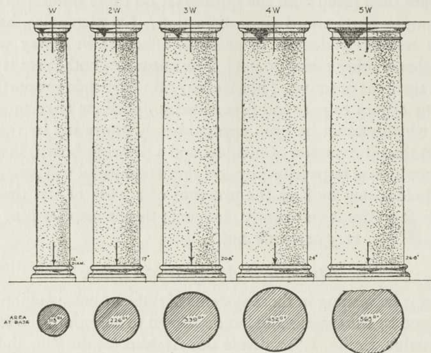
FIG. 45. Conventional columns, modified as to area only, in proportion to a series of increasing loads.
