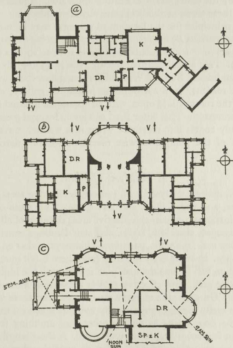
FIG. 118. Three types of house planning for prospect and aspect.
