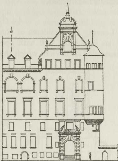
FIG. 148. New Scotland Yard, London (Norman Shaw). A masterly marshalling of irregular window groups.
