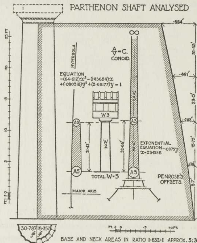
FIG. 74. Taper and entasis of the Parthenon shaft.
