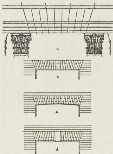
FIG. 64. In the voussoired flat arch the effect is contrary to what might be expected; see text.
