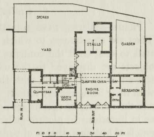
FIG. 125. Highbury Fire Station, London; 1905. (L.C.C. Architect.)
