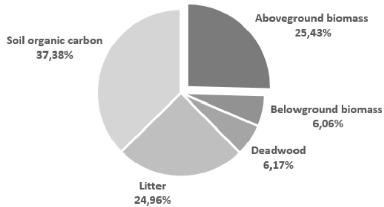
Figure 3. Distribution of Carbon stocks in FMU 073-51 calculated using Silvilib.
