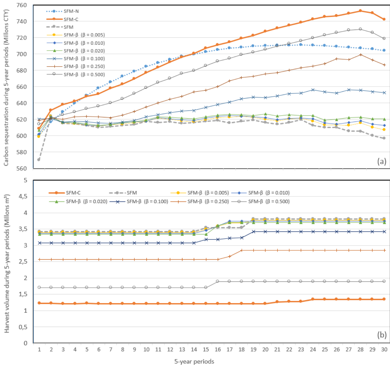
Figure 4. Carbon sequestration (a) and harvest volume (b), for each 5-year period in (Millions m 3 ) as calculated using nine alternative strategic management models.
