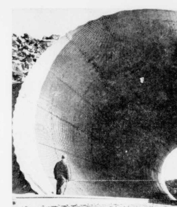
IT'S REALLY BIG. This huge culvert, largest of its kind in the United States and possibly the largest in the world, enables trucks to pass overhead without interfering with rail shipments below. The 190-foot-long pipe is 30 feet in diameter and weighs about 200 tons. It was installed recently at Cleveland Cliffs Iron Company's Palmer, Mich., plant.
