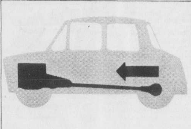
TRACTION ARRIERE
