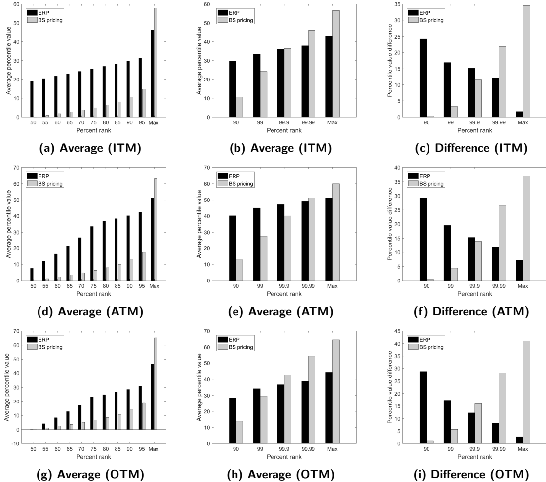
Figure 3: Comparison of hedging performance achieved under the Black-Scholes and the equal risk pricing of a European call option with K = 16 rebalancing periods under a worst-case risk measure that accounts for \mathcal{U}_2 . (a),(d), and (g) present for different percentile ranks q , the average among the q -percentile of the loss incurred for the writer and buyer of the ITM, ATM, and OTM options respectively. (b),(e), and (h) presents similar information but focusing on higher percentiles. (c), (f), and (i) present the difference between the same q -percentile losses. Note that the "Max" rank refers to the worst-case sample path.
