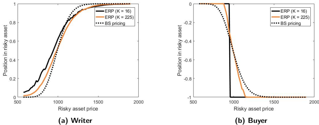
Figure 4: Comparison of hedging strategies for a European ATM Call option under different number of rebalancing periods. (a) presents the optimal strategies for the writer under the Black-Scholes and the equal risk pricing models for time k = 0 . (b) presents the same for the buyer.
