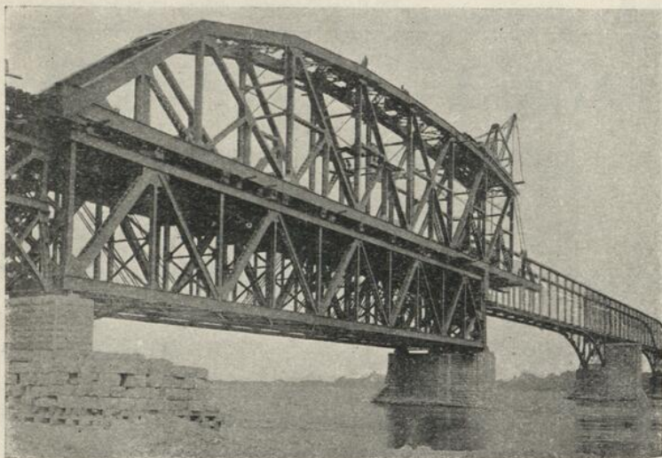
Bridge over the St. Lawrence River at Lachine, P. Q.
