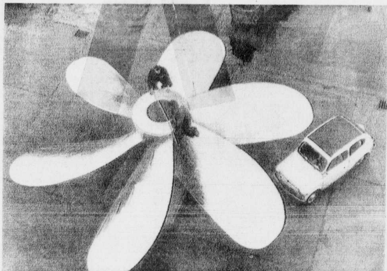
PLENTY OF DRIVE — Workmen but finishing touches to a 28-foot ship's propeller in Hamburg, West Germany, yard. The bronze-aluminum alloy screw, weighing 62 tons,
