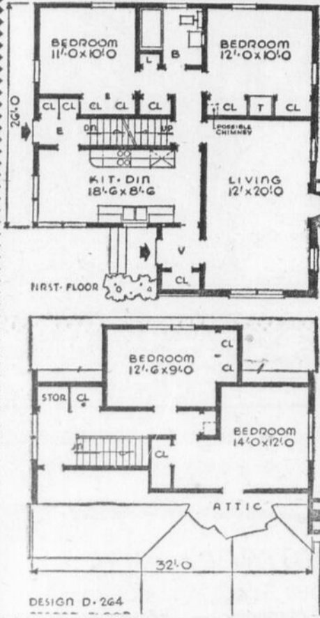
A SMALL HOUSE PLANNING BUREAU DESIGN NO. D-264
