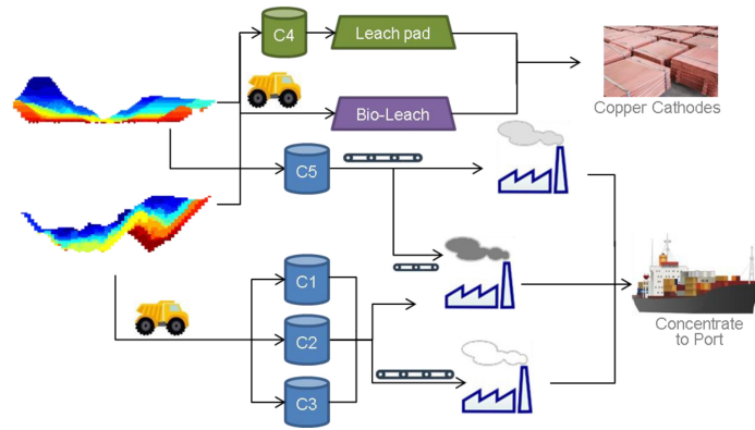
Figure 1: Schematic representation of the Escondida-Norte mining complex
