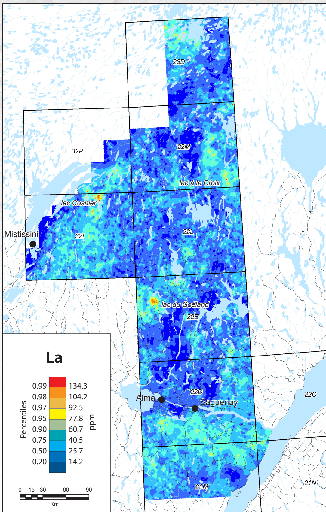
Figure 4 – Map of lanthanum anomalies in lake-bottom sediments.
