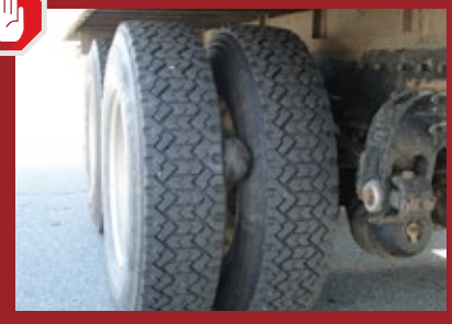
FIGURE 41 | Tire showing a bulge related to a carcass defect
