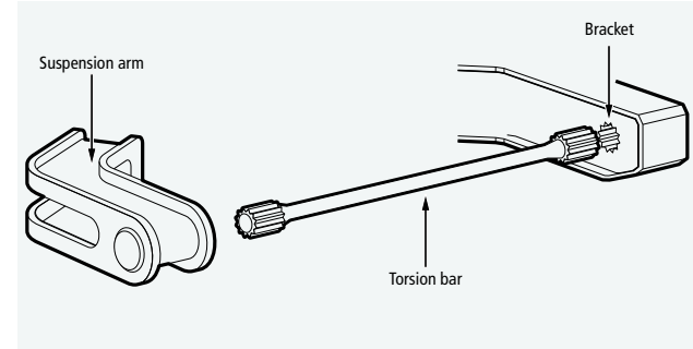
FIGURE 49 | Torsion bar
