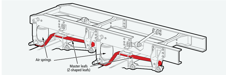
FIGURE 50 | Pneumatic suspension
