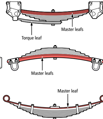
FIGURE 52 | Master leaves
