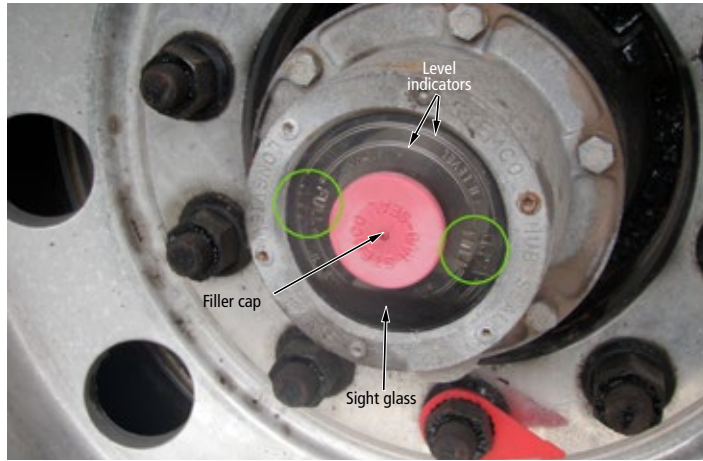
FIGURE 46 | Wheel hub sight glass
