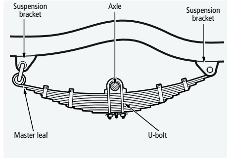
FIGURE 47 | Leaf spring
