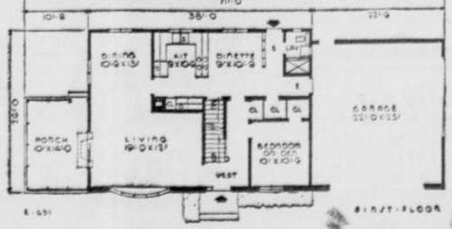
A SMALL HOUSE PLANNING BUREAU DESIGN NO. E-631
