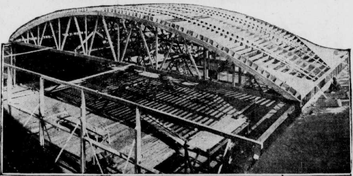
Shown in the above photo is the largest garage in Sherbrooke — Cie Cyr & Allard Ltee. This building was constructed with "Bowstring" arches or trusses. This is the ideal construction method for arenas, garages, warehouses; the cost of this type of construction in wood being 1/3 that of steel.
