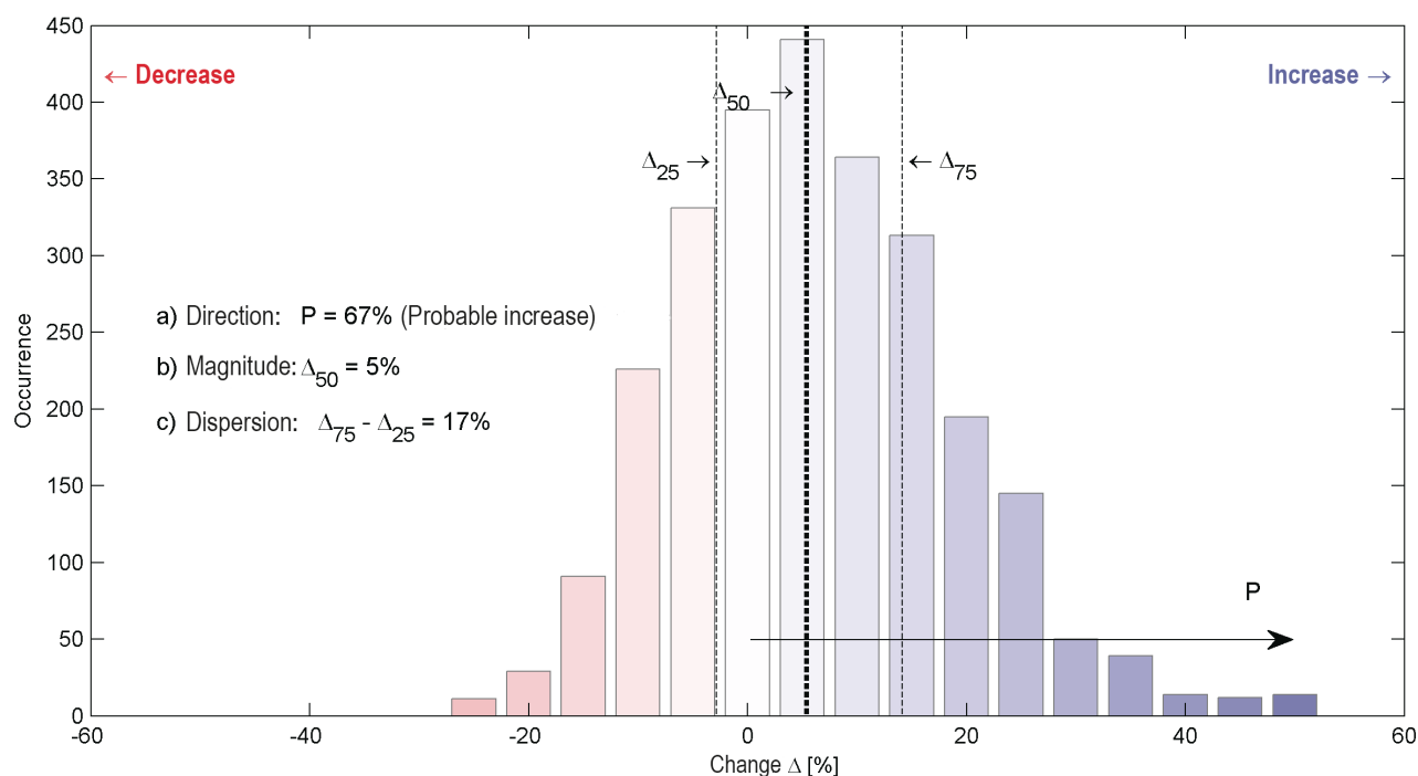
Figure 5: Hydrological change signals
