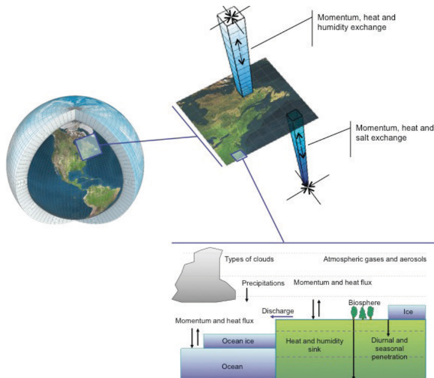
Figure 1: Schematisation of a global climate model
