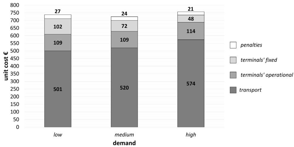
Fig. 7. Unit costs for different levels of demand.
