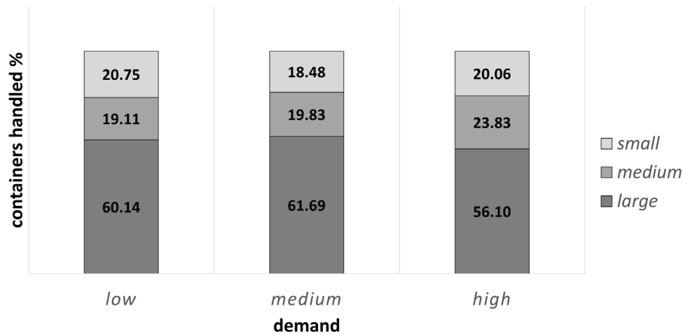
Fig. 16. Percentage of containers transhipped for each terminal size for different levels of demand.
