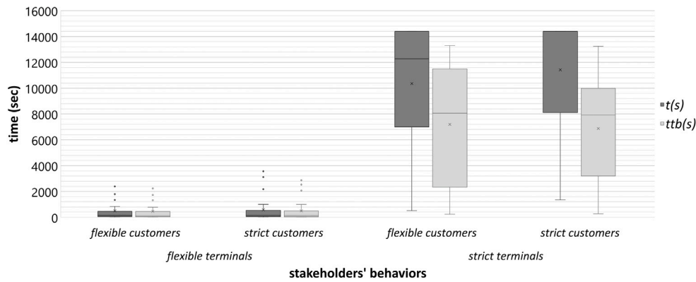
Fig. 2. t(s) and ttb(s) for flexible and strict stakeholders.
