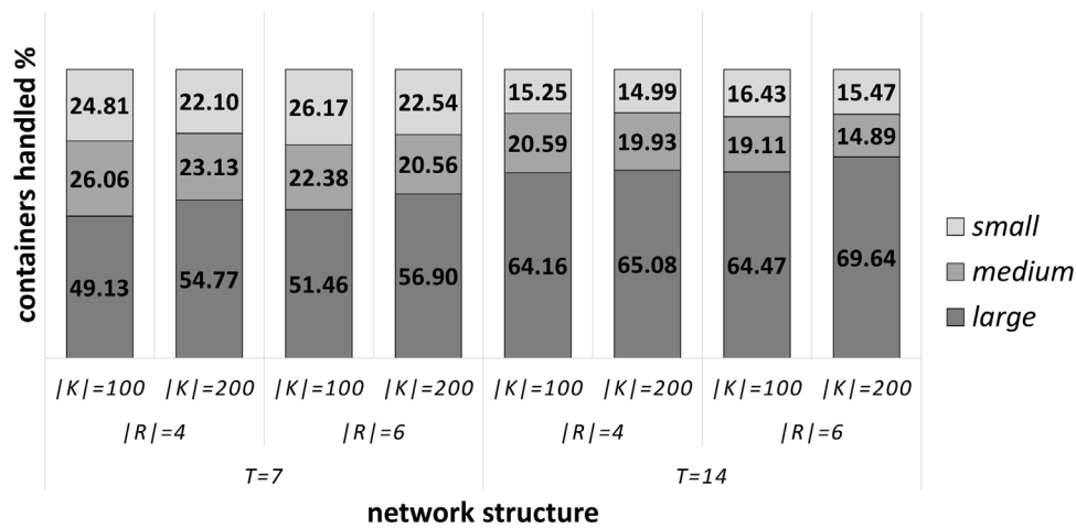
Fig. 15. Percentage of containers transhipped for each terminal size for different numbers of regions, commodities, and periods.
