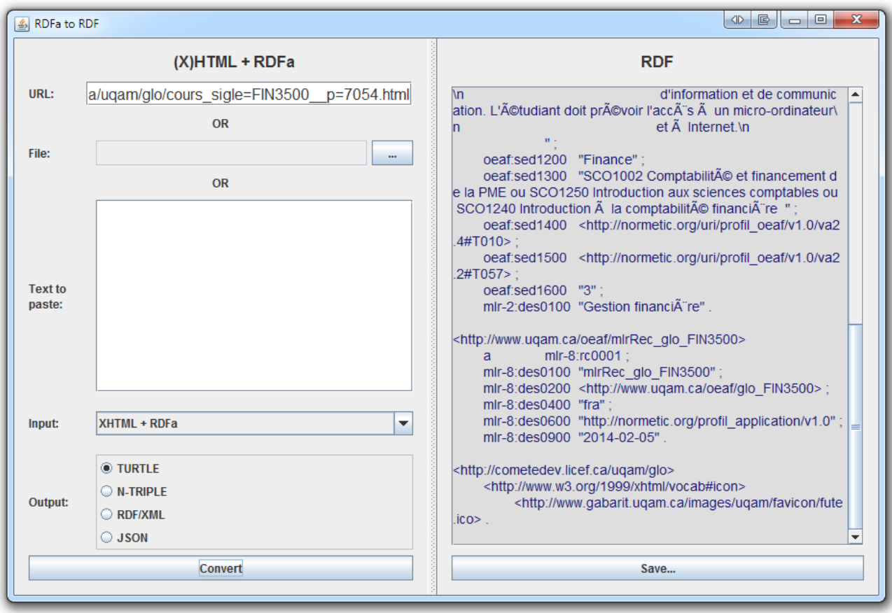
Figure 6 : Outil rdfa2rdf
