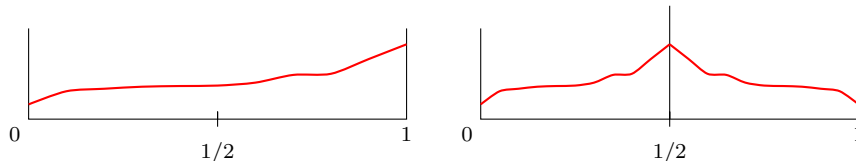
Figure 4: Applying the baker transformation to the points \mathbf{U}_i is equivalent to transforming f as shown.
