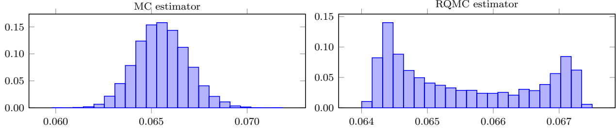
Figure 10: Histogram of MC and RQMC estimators with n = 8191 for the stochastic activity network with CMC, for x = 100 , based on m = 10000 replications of each estimator. The RQMC estimator is a randomly shifted lattice rule with n = 8191 .
