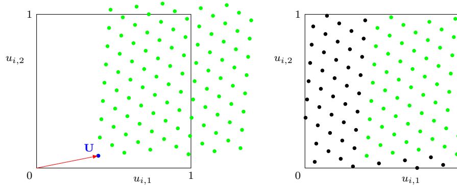
Figure 3: Random shift modulo 1 for the lattice of Figure 2 (left), with \mathbf{U} = (0.40, 0.08) .
