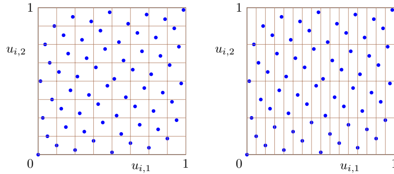
Figure 5: The Hammersley point set (or Sobol net with appended first coordinate) for s = 2 and n = 64 .
