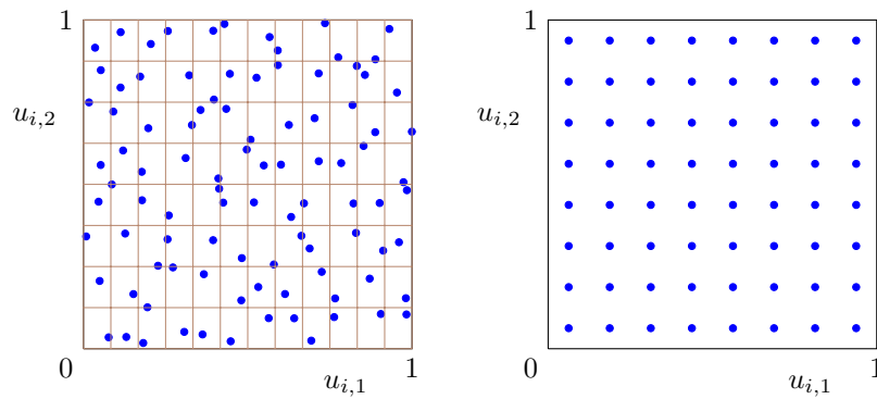
Figure 1: An illustration of stratified sampling (left) and a midpoint rule (right) over (0,1)^2 .
