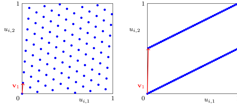
Figure 2: An integration lattice with s = 2 , n = 101 , with \mathbf{v}_1 = (1, 12)/n on the left and \mathbf{v}_1 = (1, 51)/n on the right. In both cases, we can take \mathbf{v}_2 = (0, 1) .
