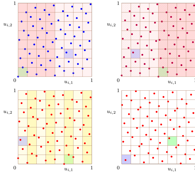
Figure 7: A random digital shift with \mathbf{U} = (0.10100101100\dots, 0.01011001100\dots)_2 applied to a Sobol net with 64 points. The original points are in upper left. Flipping the first bit of the first coordinate permutes the left half with the right one, giving the upper right plot. Then flipping the third bit of the first coordinate gives the lower left plot. The lower right shows the points after the full digital shift of the two coordinates. One can follow the movement of the green and blue boxes during the permutations. In the end, those two square boxes are permuted.
