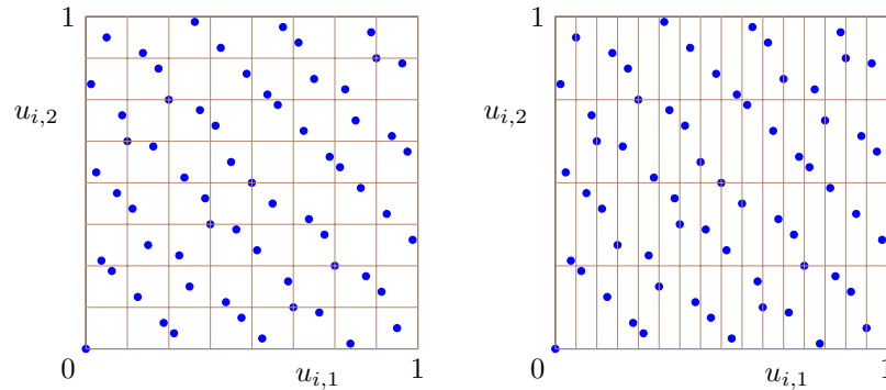
Figure 6: The first n = 64 Sobol points in s = 2 dimensions.
