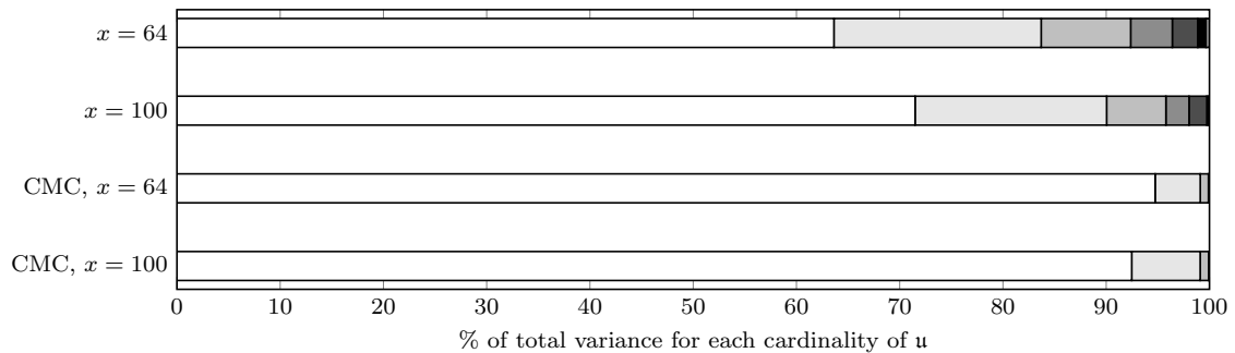
Figure 9: ANOVA Variance captured by each projection order for estimators of \mathbb{P}[T > x] for the stochastic activity network example.
