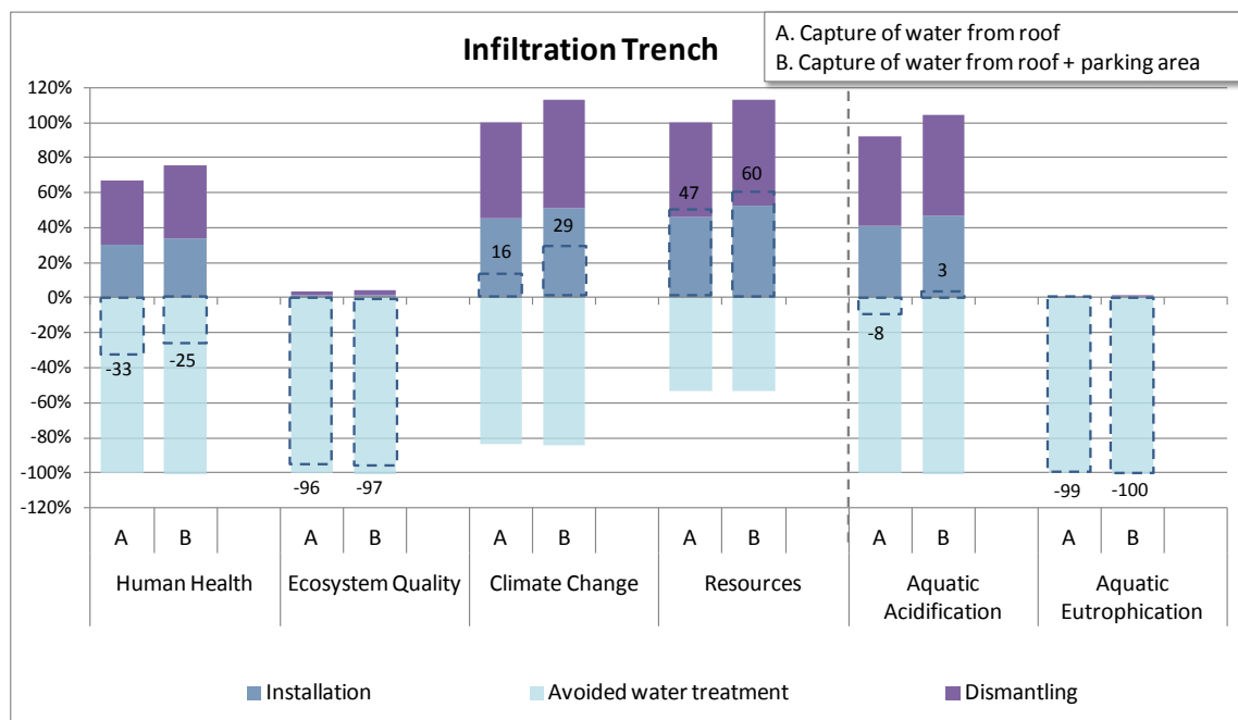
Figure 3-7: Comparison of an infiltration trench compared to the baseline scenario
