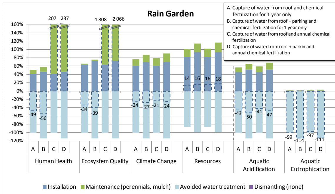
Figure 3-6: Comparison of a rain garden with the baseline scenario
