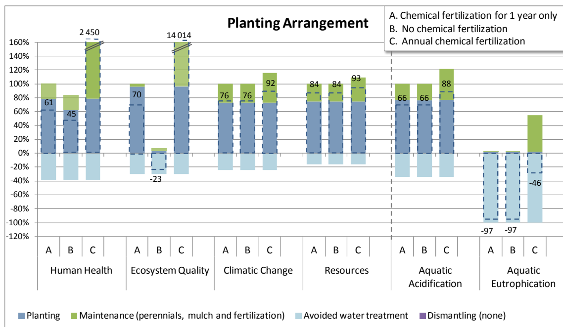
Figure 3-3: Comparison of a planting arrangement with the baseline scenario
