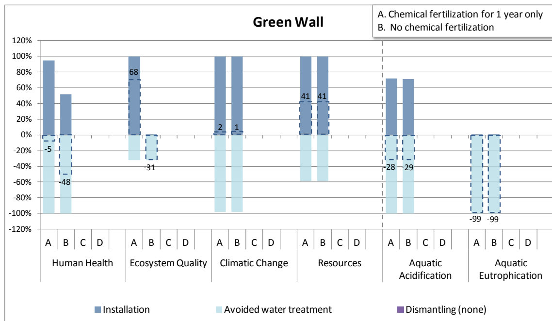
Figure 3-2: Comparison of a green wall with the baseline scenario
