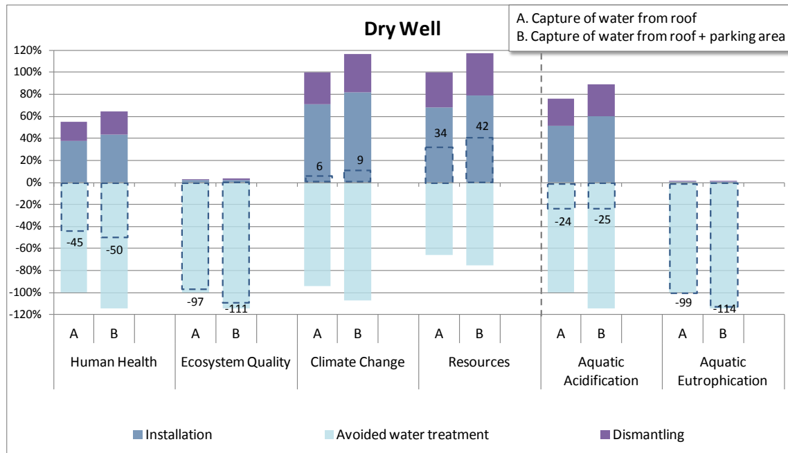
Figure 3-8: Comparison of a dry well compared to the baseline scenario
