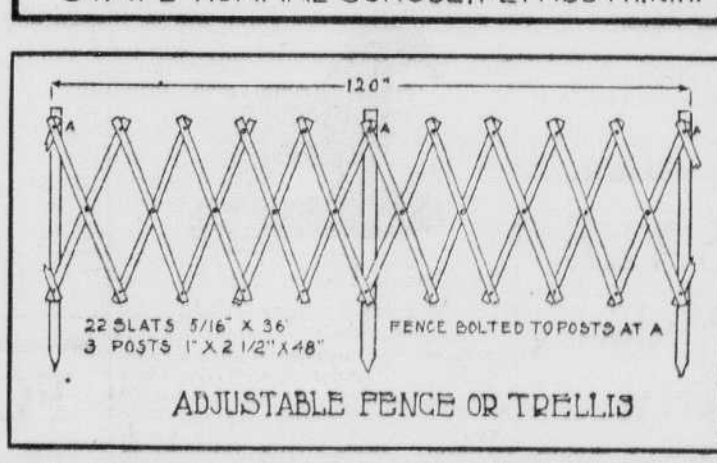
ADJUSTABLE FENCE OR TRELLIS
