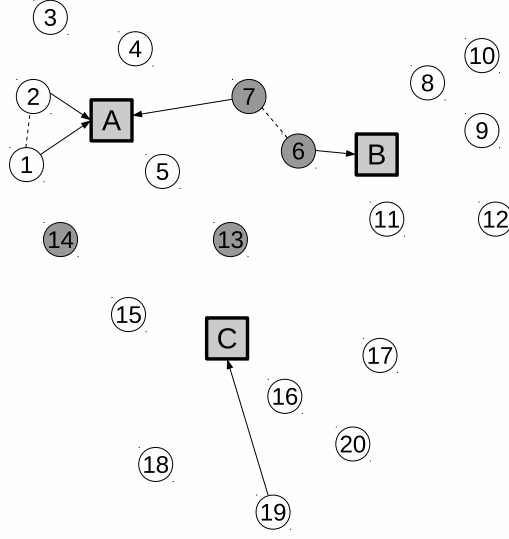
Figure 3: Problem decomposition: Assignment of customers to depots.
