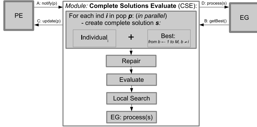
Figure 8: Complete Solutions Evaluate module.
