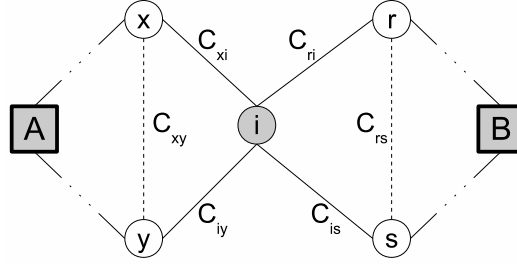
Figure 9: Repair procedure – remove duplicates
