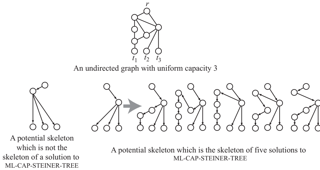
Figure 2: Potential skeletons in a graph G .
