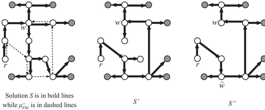
Figure 8: Illustration of the proof of Claim 7.
