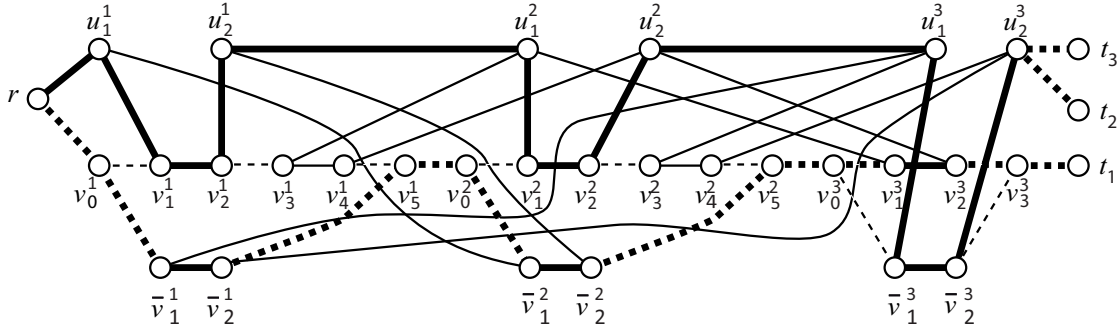
Figure 6: From SAT to CAP-STEINER-TREE.
