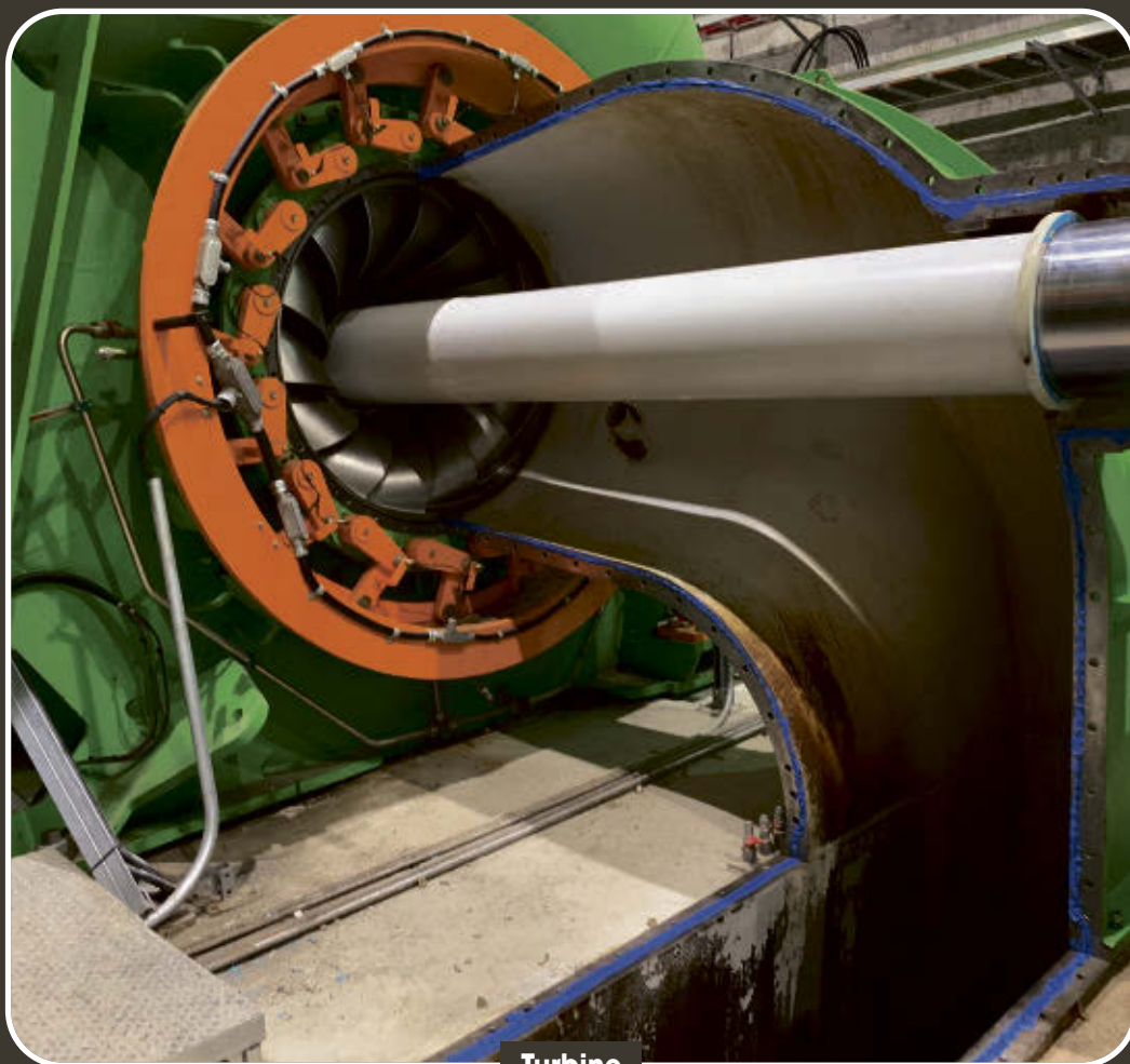
Turbine
