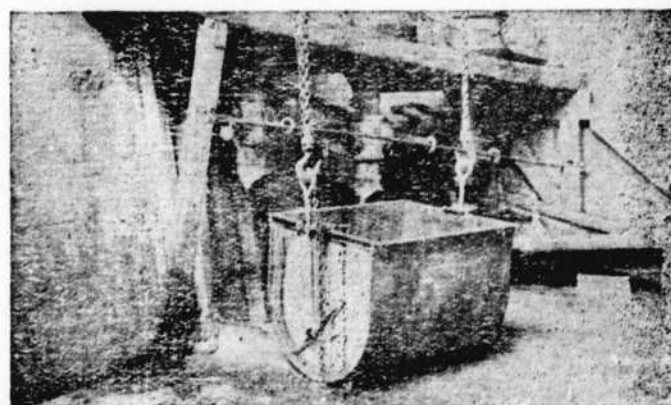
Hydraulic concentrating cones in Siscoe mill. Every two hours these cones are tapped and the resulting high grade concentrate is caught in the iron bucket shown
