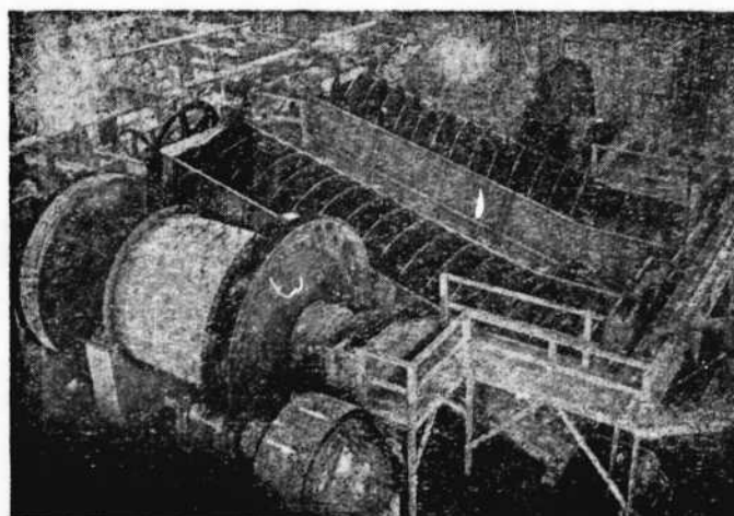
Allis-Chalmers grinding unit at the East Malartic Gold Mines Broyeurs Allis-Chalmers (Studio Morasse, Amos)
