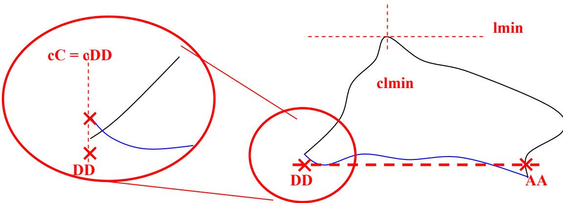
Figure 42 - if c_{AA} < c_B and c_{DD} > c_C : Definition of the second and third interpolation segments
