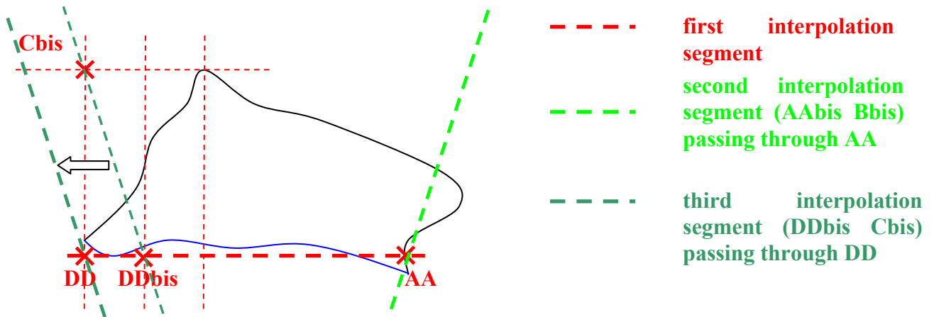
Figure 45 -- if cAA > cB or cDD < cC : Definition of second and third interpolation segments
