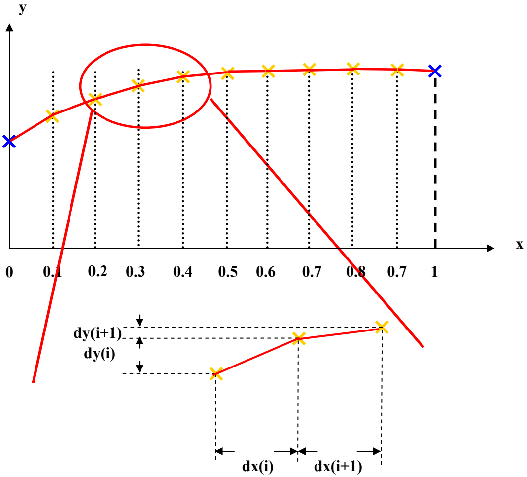
Figure 35 - Second derivative calculation method
