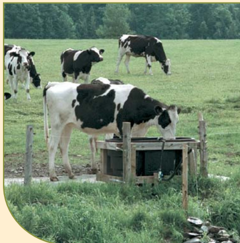
450 L (100 GALLON) TANK WITH THE OVERFLOW DISCHARGING INTO THE STREAM.
