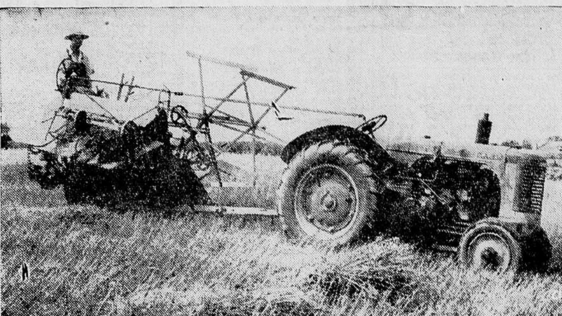
ONE-MAN GANG —Bradley Rutherford has worked out a way to operate the binder and tractor pulling the binder by himself on his farm near Stratford, Ont. He installed a steel shaft from the steering wheel of the tractor to a home-made steering wheel on the binder. A small rope from the tractor to the binder allows him to operate the hand clutch. He completed most of his harvest single-handed and quickly. (CP Photo)
