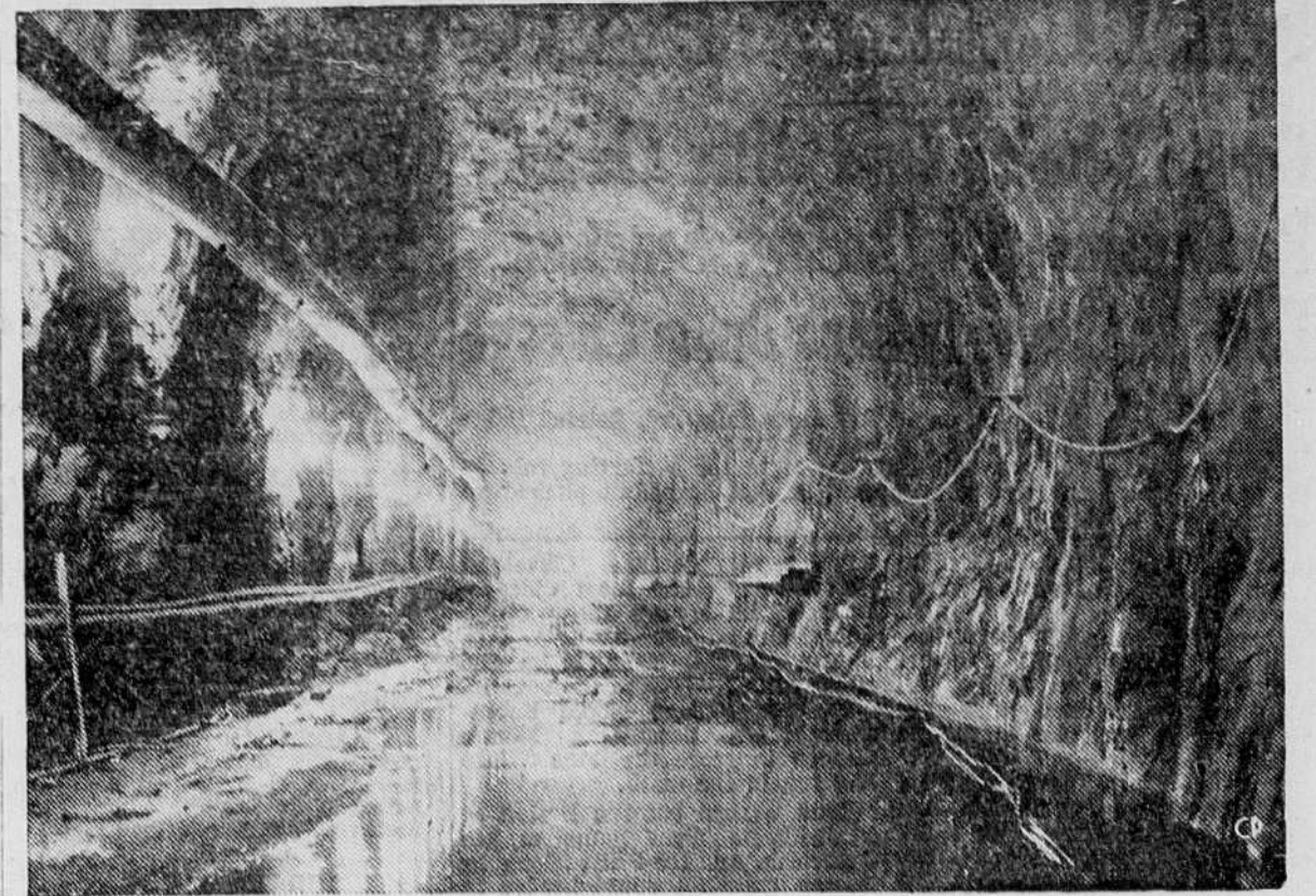
POWER TUNNEL —This tail-race tunnel, which channels water into the Kemano River, is one of a series built through the coast mountain range for the $550,000,000 aluminum industry under construction at Kitimat, B.C., 450 miles north of Vancouver. Water is backed up from the Nechako dam to create a 350-square-mile watershed and is carried through a tunnel to the power site 125 miles west of the dam. The water then is carried off through a tail-race tunnel to the Kemano River which joins the Pacific ocean at Gardiner Canal. (CP Photo)
