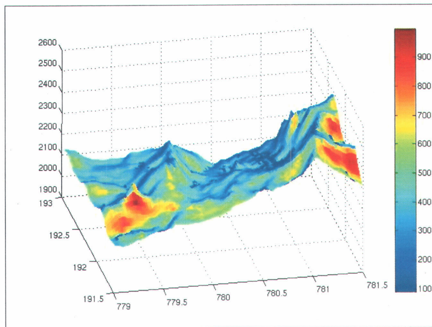
Figure 4 - Incoming shortwave radiation on the 15 th of January, 2003 at 12 p.m.
