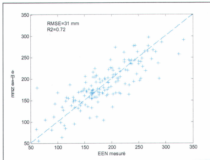
Figure 2 - Comparison of estimated and measured Snow Water Equivalent.
