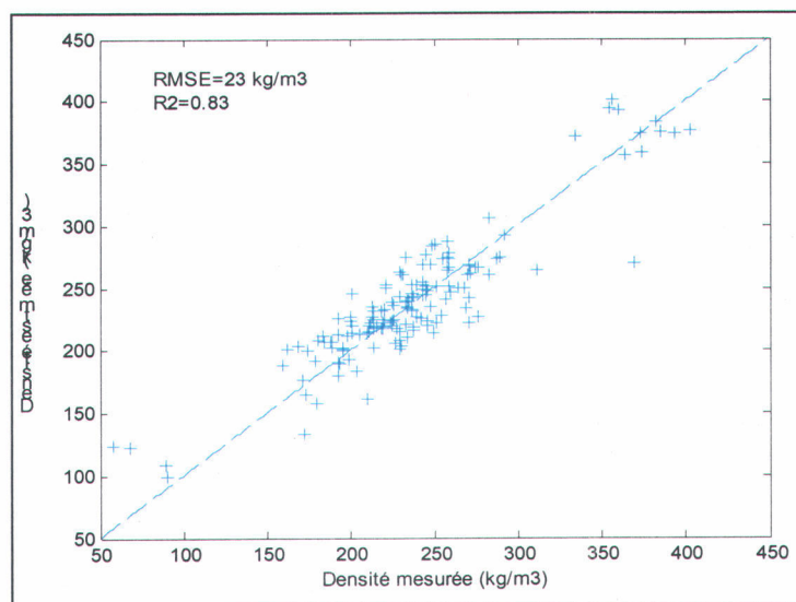
Figure 1 - Relationship between estimated and measures snow density
