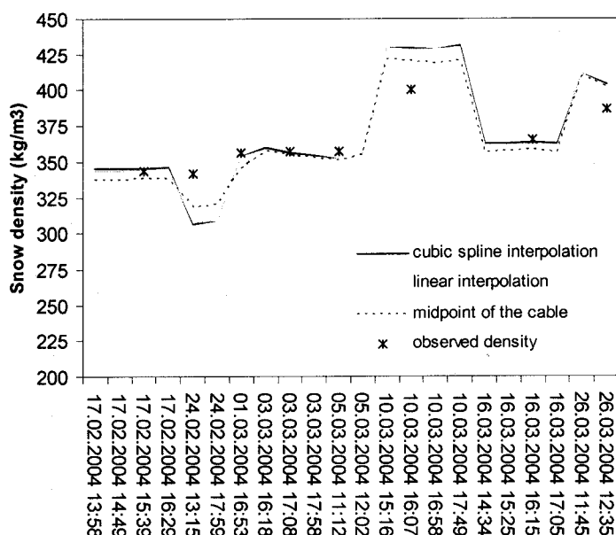
Figure 22 - Simulated snow densities using the three methods of temperature calculation and compared with manual observations. \alpha=0.3333 .
