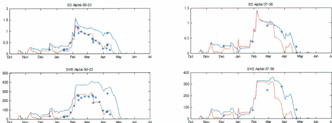
Figure 5 - Simulated (lines) and manually measured (dots) snow depth (top) and SWE (bottom) for two selected sites in the Alptal catchment: a site with weekly measurements (left) and a site with monthly measurements (right). The blue line shows the simulation without snow updating, and the red line represents a simulation with the updating routine.
