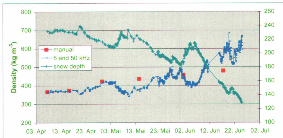
Figure 14 - Comparison of BSI density measurements (based on 6 and 50 kHz) with manual reference measurements together with snow depth measurements (in cm) at the Swiss test site.
