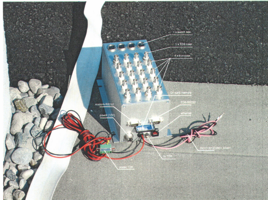
Figure 8 - BSI with IA-module, Multiplexer and option for TDR module connection
