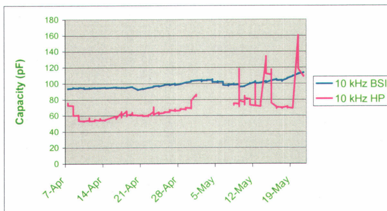
Figure 12 - Comparison of measured capacities at 10 kHz of BSI with laboratory set-up (HP) at the Swiss test site.
