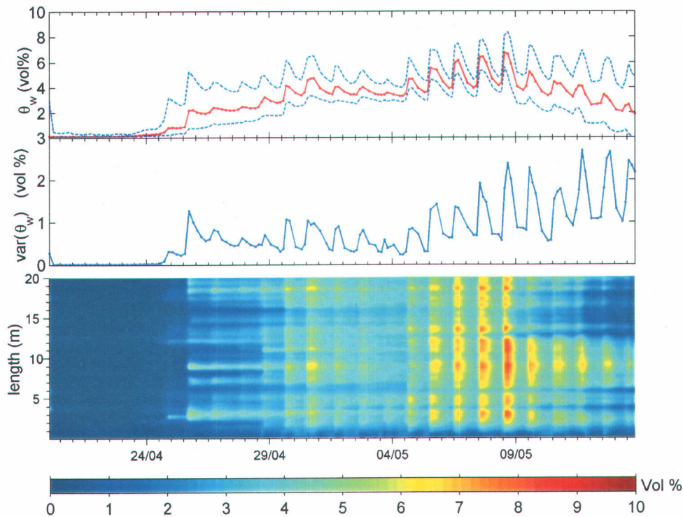
Figure 16 - Preferential flow patterns detected with the high frequency (TDR) measurements of the SNOWPOWER sensor.
