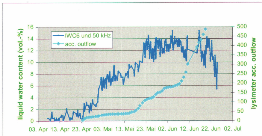
Figure 15 - Comparison of liquid water content measurements from the BSI prototype (based on 6 and 50 kHz) with accumulated outflow of the lysimeter at the Swiss test site.
