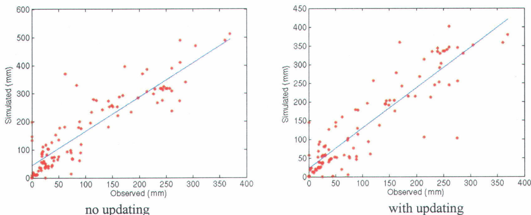
Figure 6 - Simulated versus manually measured SWE (mm) for 15 locations in the Alptal catchment during winter 2002/03.
