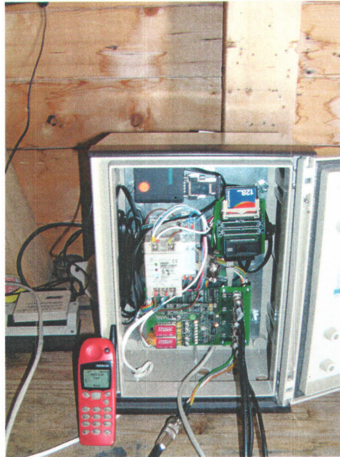
Figure 7 - BSI at the Swiss test site in the weather-proof installation box
