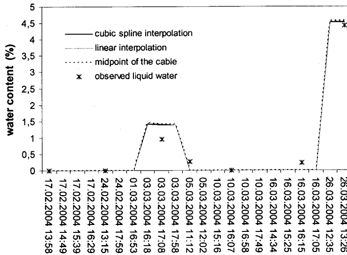
Figure 23 - Simulated snow liquid water content using the three methods of temperature calculation and compared with manual observations. \alpha=0.3333 .
