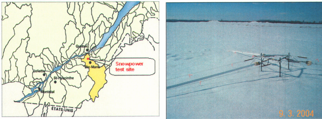
Figure 17 - Test-site localisation and SNOWPOWER cable installation at the agricultural field
