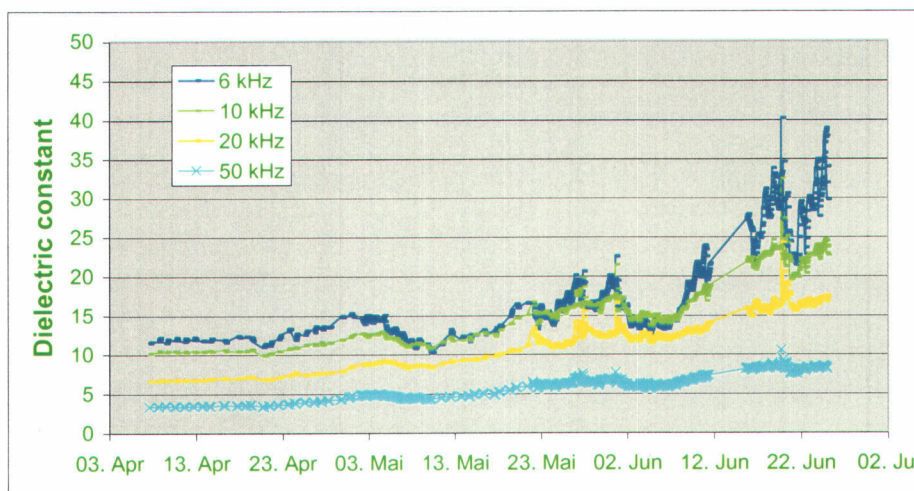
Figure 13 - Dielectric constants at low frequencies (6, 10, 20, 50 kHz) determined with BSI at the Swiss test site
