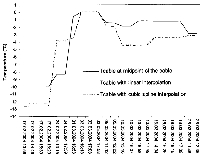
Figure 19 - Comparison of the three methods of temperature calculation
