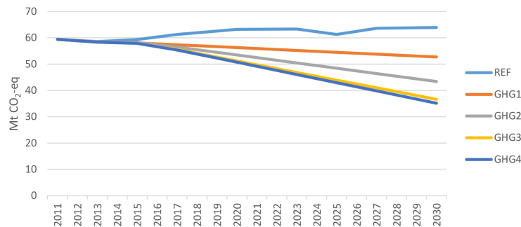
Figure 1: Total GHG emissions from the energy sector in Quebec
