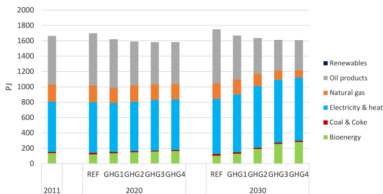
Figure 3: Final energy consumption by fuel in Quebec * Renewables include decentralized geothermal and solar energy of the residential and the commercial sectors.
