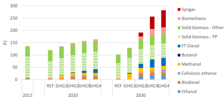
Figure 6: Bioenergy consumption by type in Quebec
