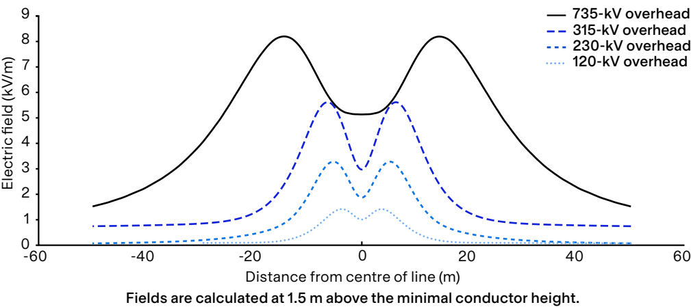
Electric field generated by HVPLs (kV/m)
