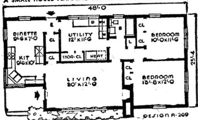
A SMALL HOUSE PLANNING BUREAU DESIGN NO. A-269
