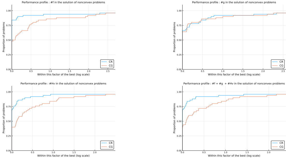
Figure 2: Performance of linesearch CR and CG on 58 nonconvex problems in terms of evaluations of f , g and products with H .
