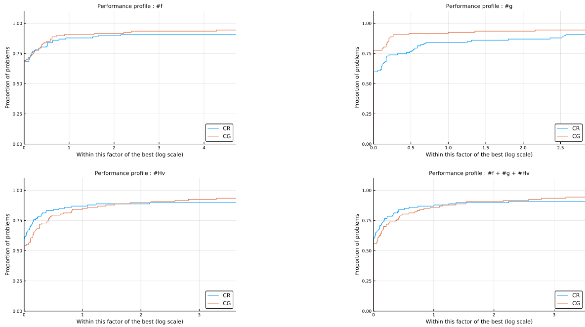
Figure 3: Performance of linesearch CR and CG on 98 problems in terms of evaluations of f , g and products with H .
