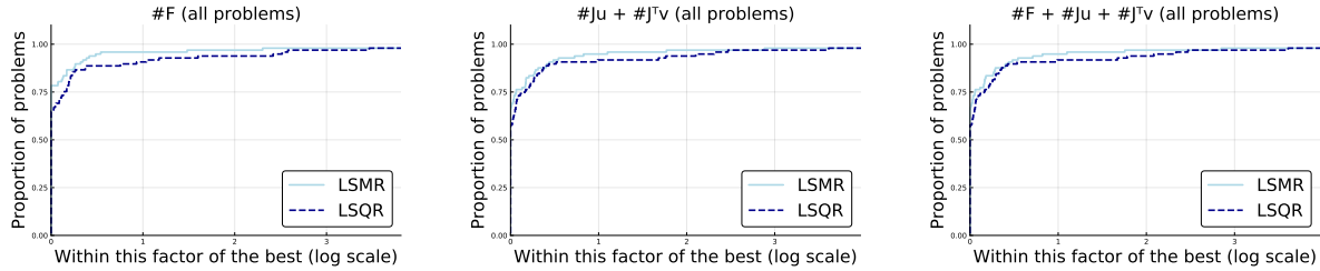
Figure 7: Performance of trust-region LSQR and LSMR on 97 nonlinear least-squares problems in terms of \#F , \#Ju + \#J^T v , and the sum of both.
