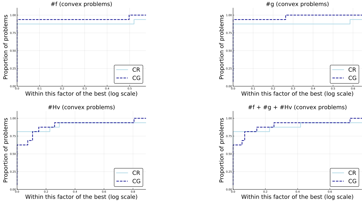
Figure 1: Performance of linesearch CR and CG to solve 16 convex problems in terms of evaluations of f , g and products with H .
