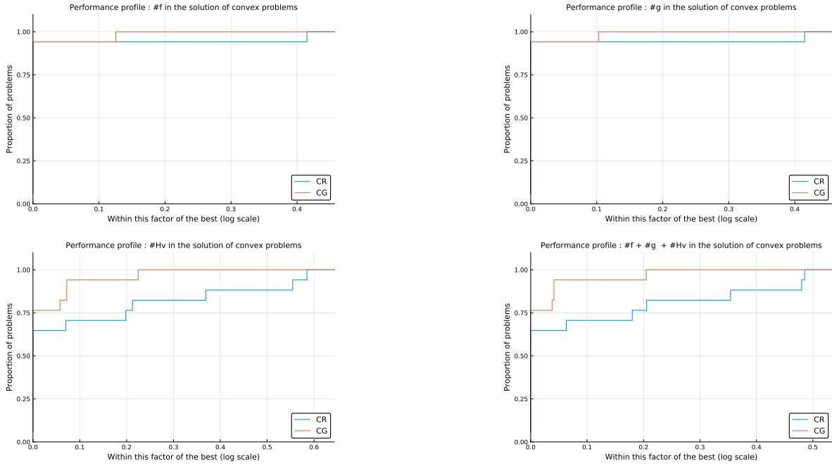
Figure 4: Performance of trust-region CR and CG on 16 convex problems in terms of evaluations of f , g and products with H .
