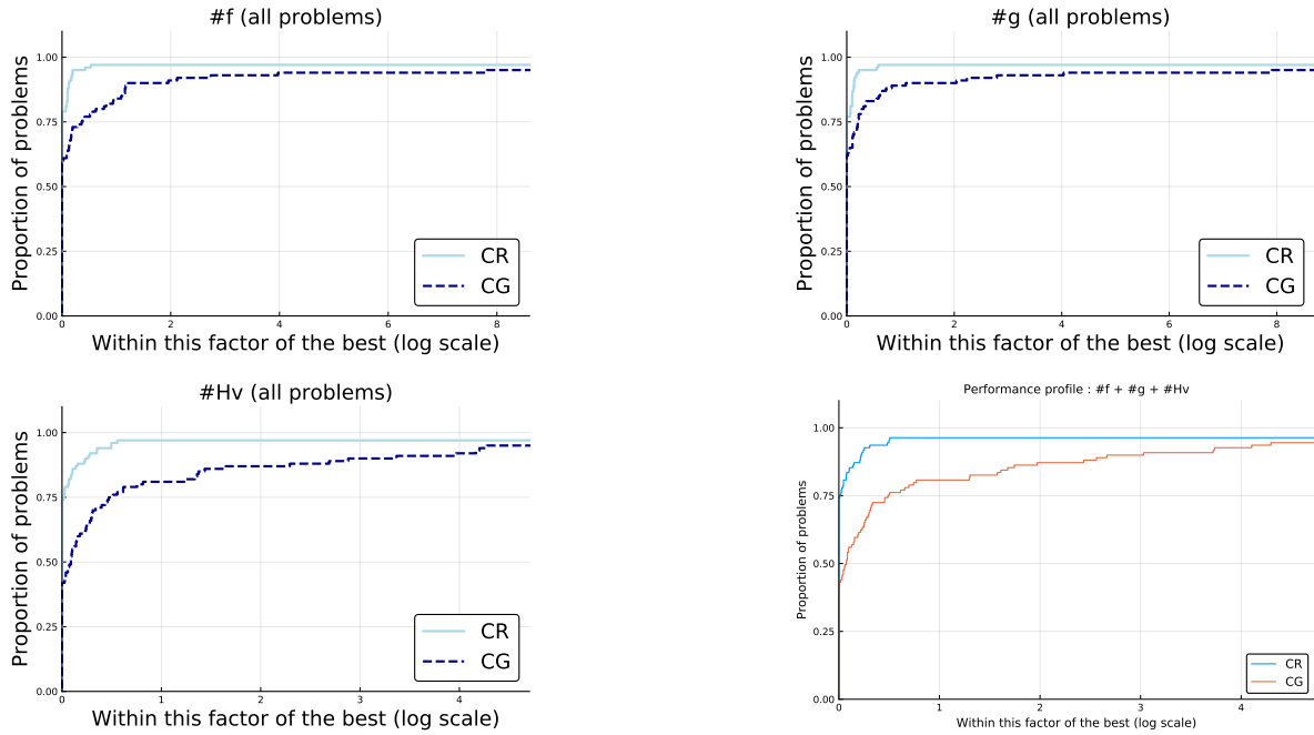
Figure 6: Performance of trust-region CR and CG on 100 problems in terms of evaluations of f , g and products with H .
