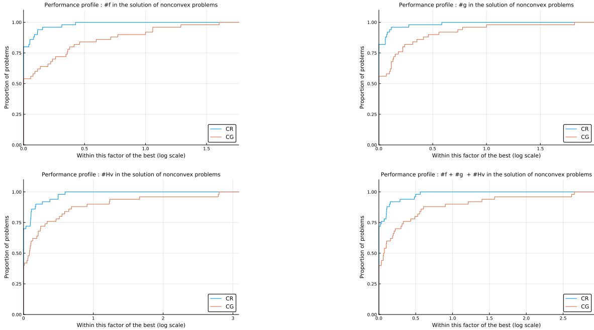
Figure 5: Performance of trust-region CR and CG on 59 nonconvex problems in terms of evaluations of f , g and products with H .
