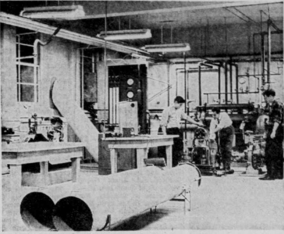
THERMO-DYNAMICS LABORATORY — Steam-power generation is facilitated by operational equipment such as shown in this photo, a few of the many pieces of industrial aid used in training engineers at the University.
