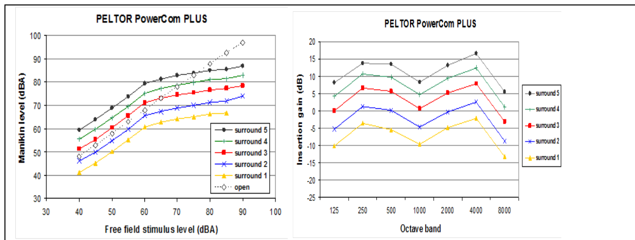
Figure 6 – PELTOR PowerCom Plus: input/output curves in a noise spectrum of speech (left) and insertion gain according frequency function in response to pink noise of 60 dBA (right)
