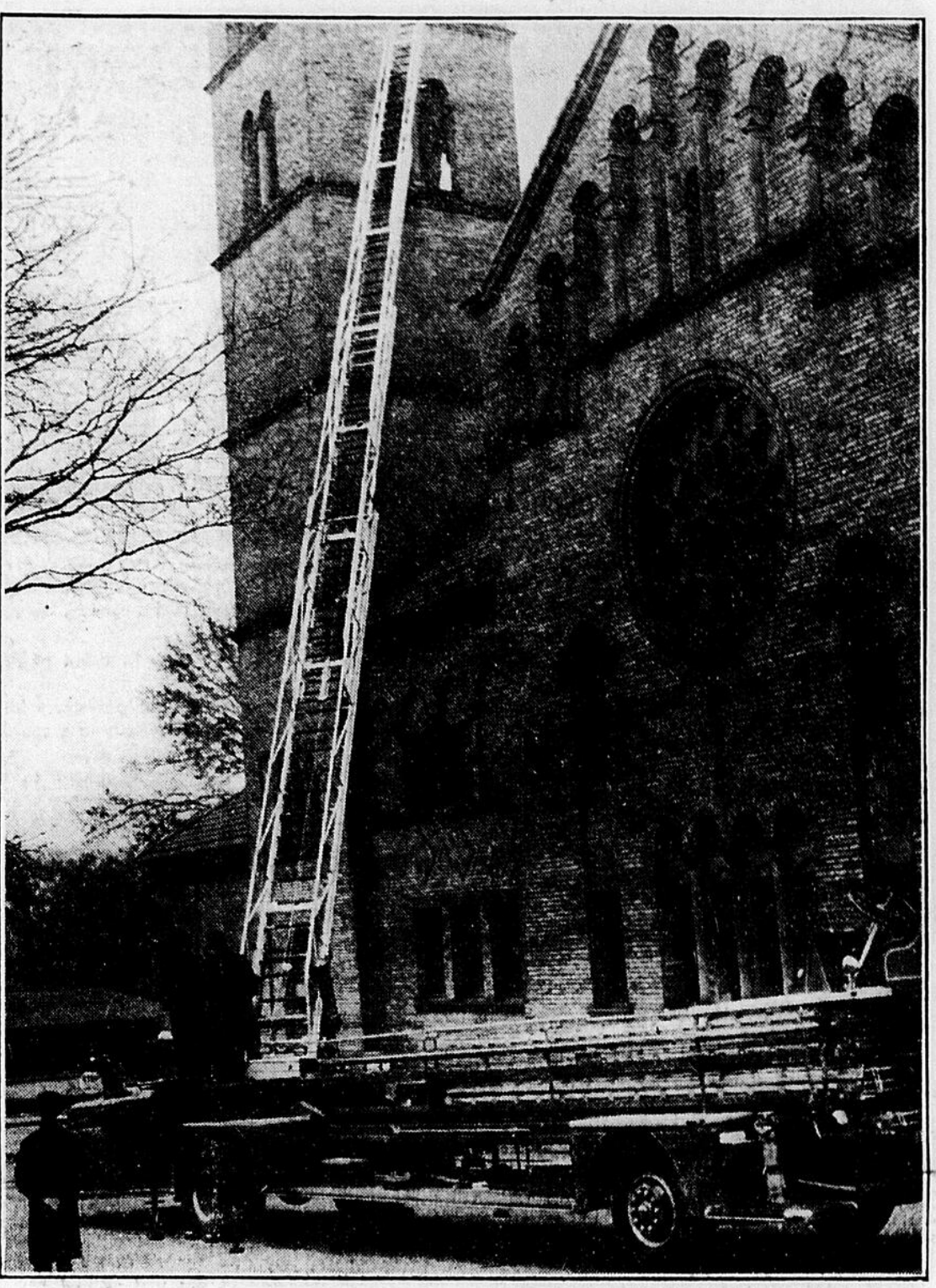
The last word in fire fighting apparatus, the 100-foot aerial ladder truck shown above was tested on Tuesday by the Westmount Police and Fire Department which is shortly to purchase a machine of this type. The motor-powered extension ladder is shown rising almost to the top of the high spire of St. Andrew's United Church, corner of Cote St. Antoine road and Stanton avenue, as the machine underwent preliminary tests. Chief Walter Gough (left), and Deputy Fire Chief Burris are standing on the ladder's control platform.
