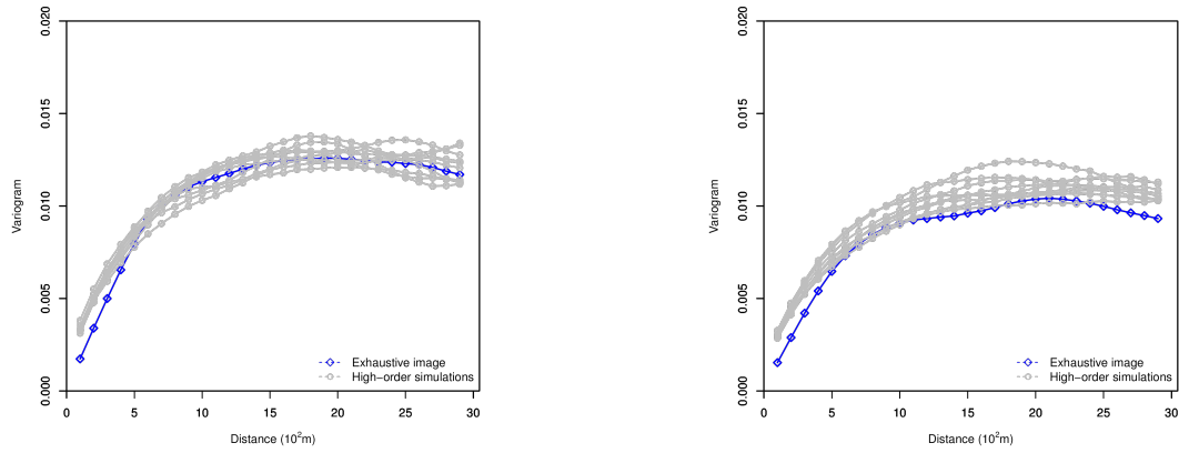
(a) Reproduction of variograms of high-order simulations in X direction
