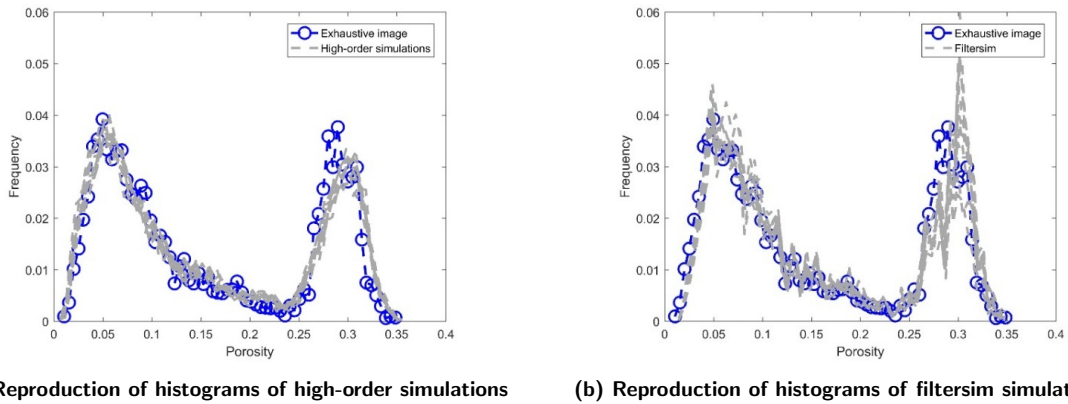
Figure 7: Reproduction of histograms of 10 realizations with 200 sample data using the exhaustive data as the training image: (a) and (b) correspond to 10 realizations from the high-order simulation and filtersim, respectively.
