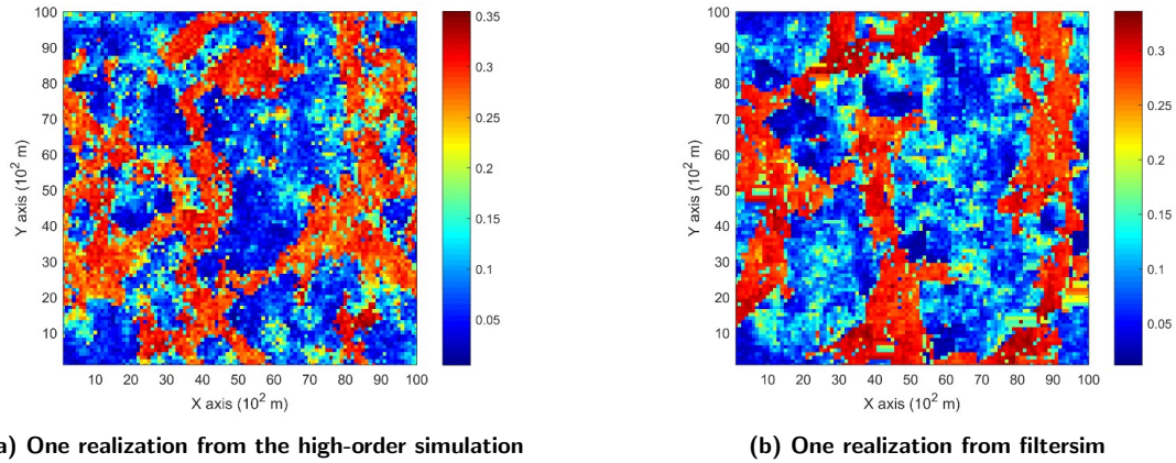
Figure 10: Simulations with 200 sample data using a separate training image different from the exhaustive data. one realization from (a) high-order simulation and (b) filtersim.
