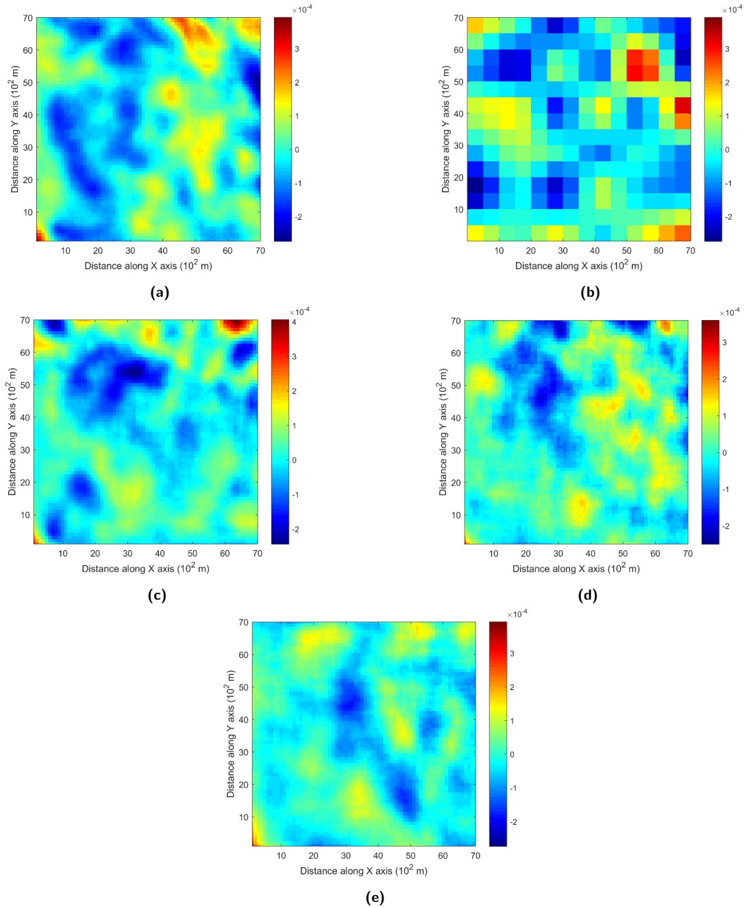
Figure 13: Third-order cumulant maps of (a) exhaustive image, (b) sample data, (c) TI, (d) high-order simulation and (e) filtersim.
