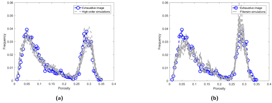
Figure 11: Reproduction of histograms of 10 realizations with 200 sample data using the training image different from the exhaustive data: (a) and (b) correspond to 10 realizations from high-order simulation and filtersim, respectively.
