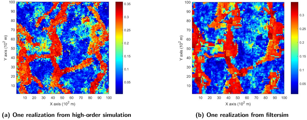
Figure 6: Simulations with 200 sample data using the exhaustive data as the training image. one realization from (a) high-order simulation and (b) filtersim.
