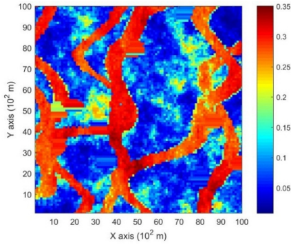
Figure 3: A horizontal section from reservoir's porosity values with sinuous connectivity.
