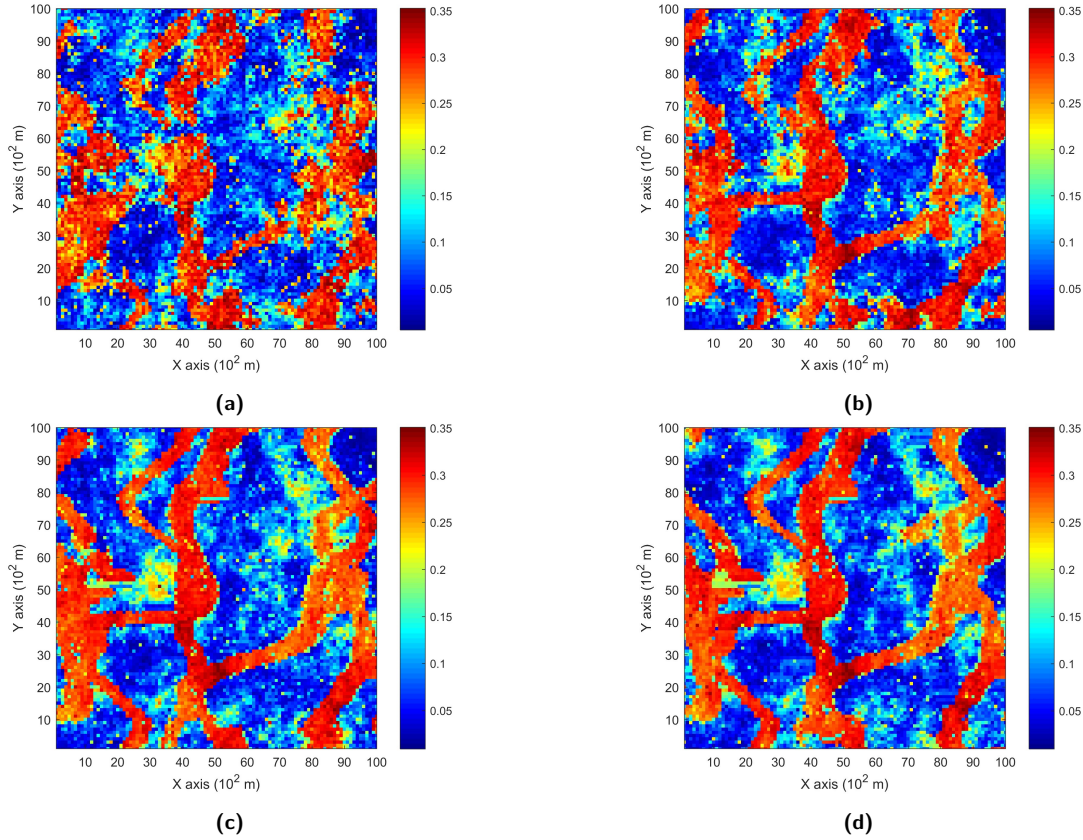
Figure 16: Comparing the realizations of the high-order simulation by applying the different order of truncated Legendre polynomial series, with 200 sample data using the exhaustive data as the training image. The number of conditioning data in the local neighborhood is 12 for all the realizations. Realizations of the high-order simulation by approximating cpdf with Legendre polynomial series up to (a) order 6, (b) order 10, (c) order 20, and (d) order 30.
