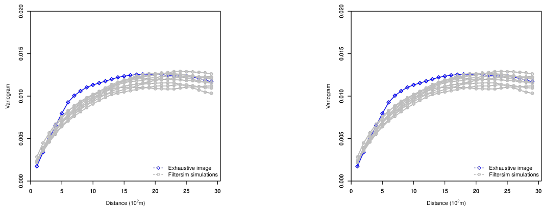
(c) Reproduction of variograms of filtersim simulations in X direction
