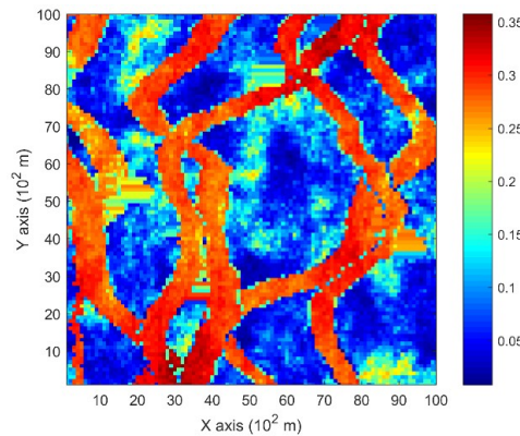
Figure 5: Training image that is different from the exhaustive data.
