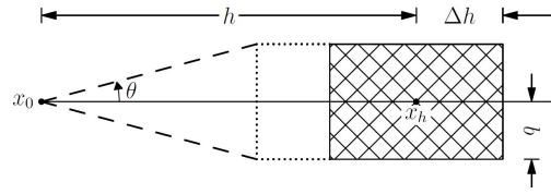
Figure 2: Finding approximate replicates from the training image with the tolerances of the original geometry template.
