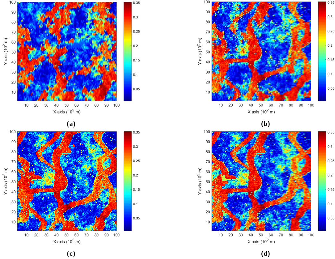
Figure 14: Comparing the realizations of high-order simulation by applying different local neighborhood size, with 200 sample data using the exhaustive data as the training image. The maximum order of Legendre polynomials to approximate the cpdfs is 10 for all the realizations. Realizations with neighborhood of (a) 6 conditioning data, (b) 12 conditioning data, (c) 20 conditioning data, and (d) 30 conditioning data.
