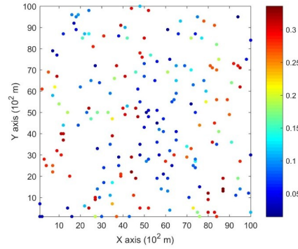
Figure 4: Data points sampled from the exhaustive image (containing 200 points, or 2% of the total data).
