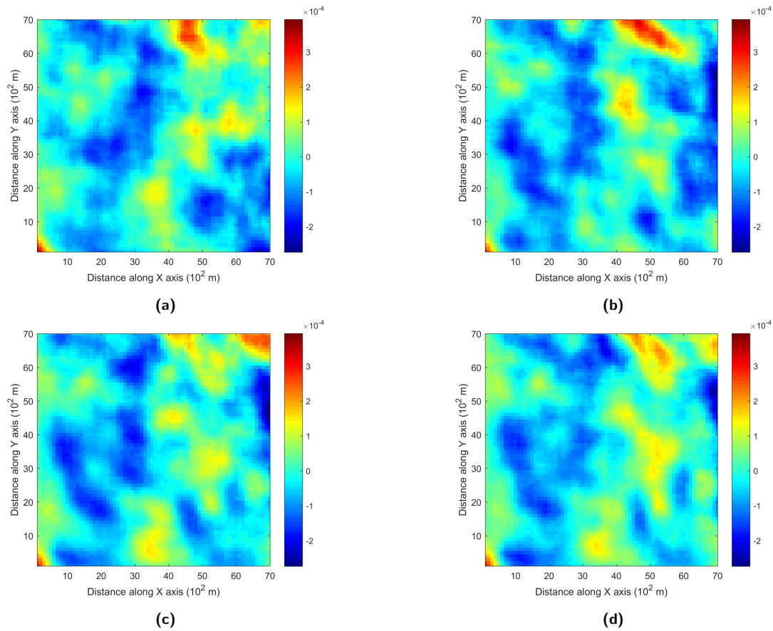
Figure 15: Comparing the third-order cumulant maps of the realizations of the high-order simulation by applying different local neighborhood size, with 200 sample data using the exhaustive data as the training image. The maximum order of Legendre polynomials to approximate the cpdfs is 10 for all the realizations. Third-order cumulant maps of one realization with neighborhood of (a) 6 conditioning data, (b) 12 conditioning data, (c) 20 conditioning data, and (d) 30 conditioning data.
