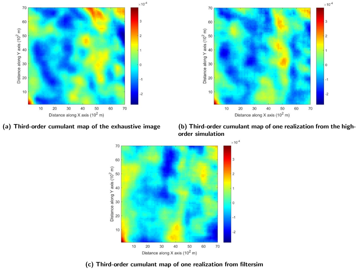
Figure 9: Comparing third-order cumulant maps of realizations with 200 sample data using the exhaustive data as the training image from the high-order simulation and filtersim, respectively.
