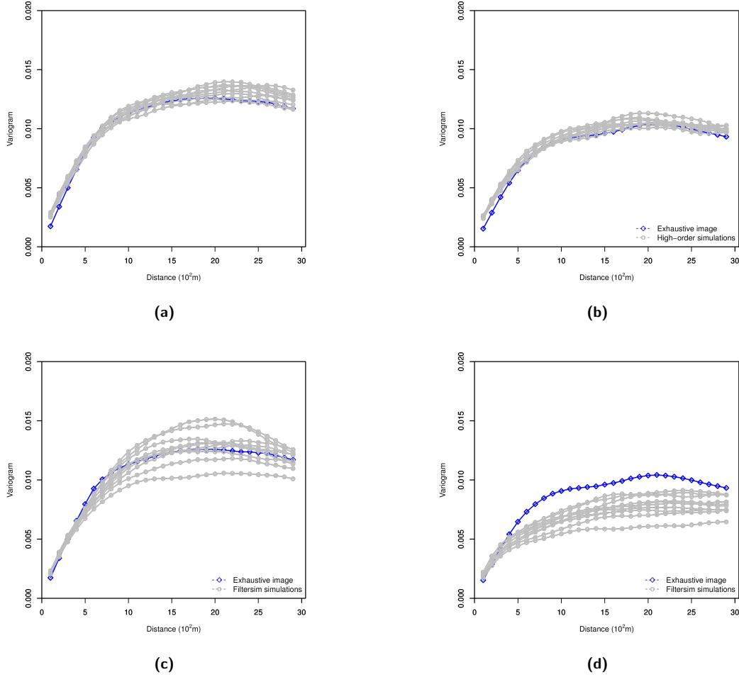
Figure 8: Reproduction of the variograms of 10 realizations with 200 sample data using the exhaustive data as the training image from high-order simulation and filtersim, respectively. (a) Reproduction of variograms of high-order simulations in the X direction; (b) Reproduction of variograms of high-order simulations in the Y-direction; (c) Reproduction of variograms of filtersim simulations in the X-direction; (d) Reproduction of variograms of filtersim simulations in the Y-direction.
