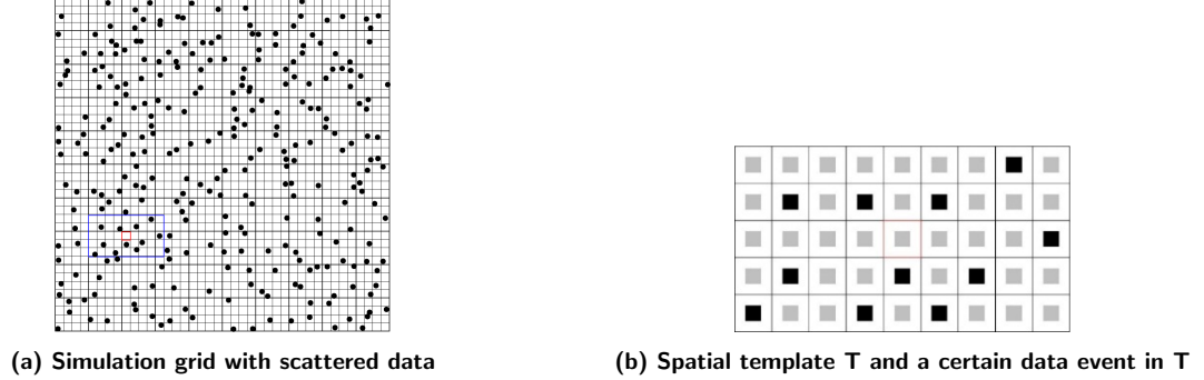
Figure 1: (a) A size 40 \times 40 grid to be simulated with a 9 \times 5 template overlaid on the current visiting node; (b) Spatial template \mathbf{T} and a certain data event in \mathbf{T} , the center square is the node to be simulated; the black squares are the conditioning data.
