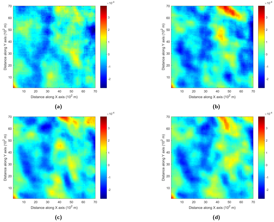
Figure 17: Comparing third-order cumulant maps of the realizations of the high-order simulation by applying the different order of truncated Legendre polynomial series, with 200 sample data using the exhaustive data as the training image. The number of conditioning data in the local neighborhood is 12 for all realizations. Third-order cumulant map of one realization of the high-order simulation by approximating cpdf with Legendre polynomial series up to (a) order 6, (b) order 10, (c) order 20, and (d) order 30.
