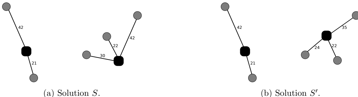
Figure 1: Example of two \alpha NpCP solutions of same cost (42).
