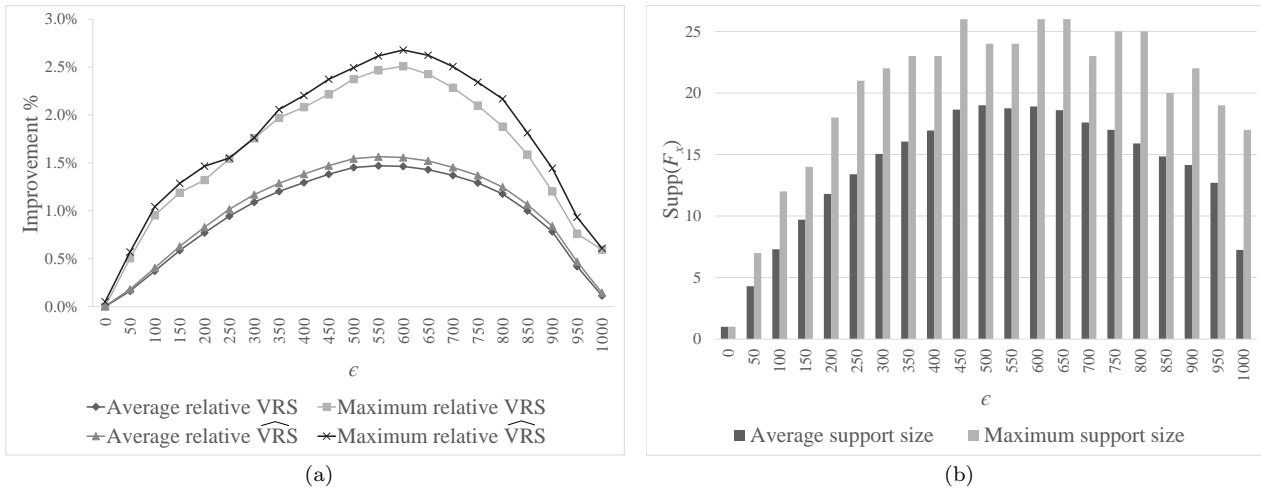
Figure 2: (a) Average and maximum \widehat{\text{VRS}} bound and actual improvement achieved by randomization. (b) Average and maximum support size of the optimal randomized strategy. Both based on 20 DRUFLP instances.
