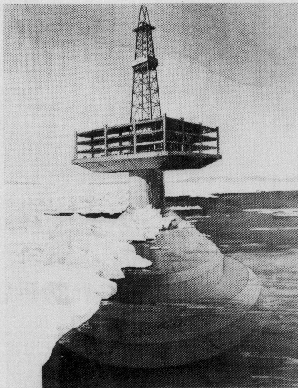
This "circular pyramid" is one of the early concepts for bringing oil up safely from beneath the Beaufort Sea. New and bolder ideas to cope with the colossal force of the Arctic icepack are still being considered by Gulf experts. Whatever the ultimate solution, hundreds of millions of dollars will be invested before a single barrel of crude can reach the consumer.
