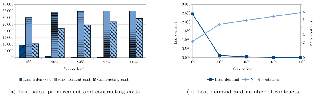
Figure 9: Results with the CRC and lost sales formulation with service level constraints
