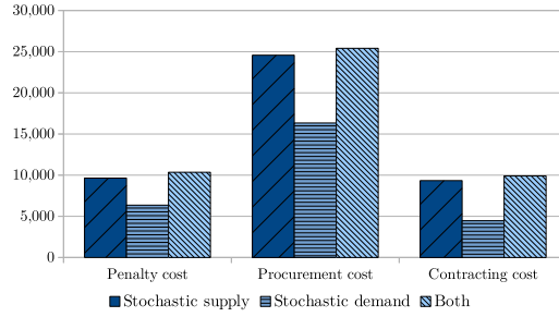
Figure 8: Results with the CRC and lost sales formulation with either stochastic supply or demand or both
