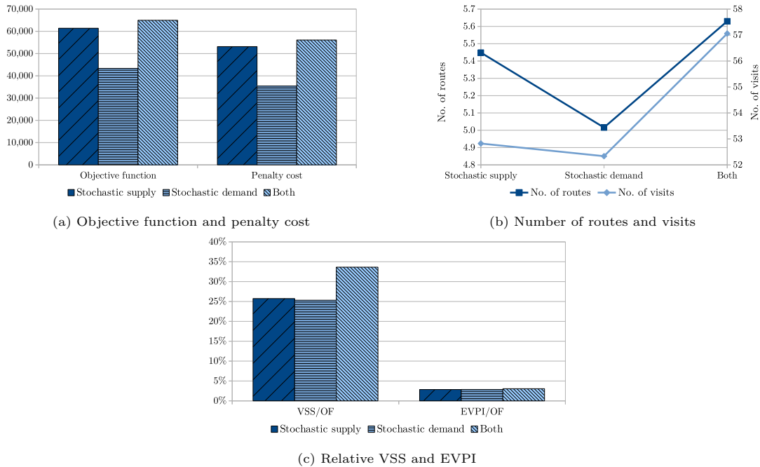
Figure 3: Results with either stochastic supply or stochastic demands or both
