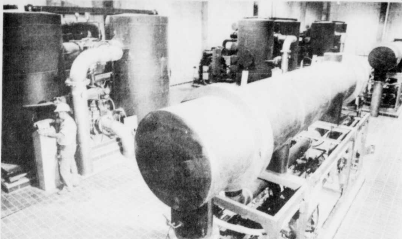
Water in the new facility is sterilized with ozone generated in these six multi-tube high-voltage discharge chambers. Ozone oxidizes organic matter in the water, sterilizing it.
