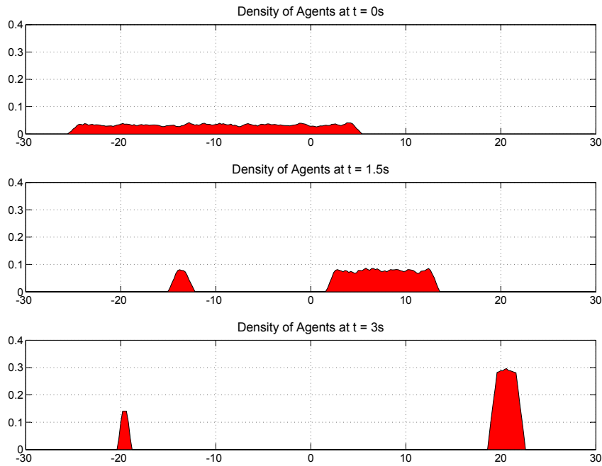
Figure 2: Evolution of the density of minor players in the presence of advertisement effect - 87% of the minor agents go towards p_2 = 20 . Under the advertisement effect, the majority of the population goes towards p_2 .
