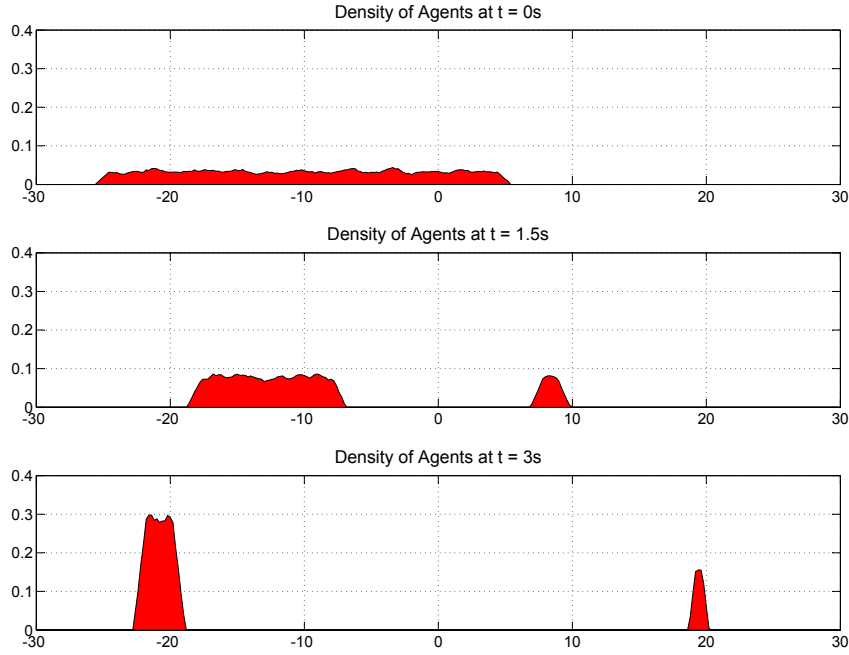
Figure 1: Evolution of the density of minor players in the absence of advertisement effect - 16% of the minor agents go towards p_2 = 20 . In the absence of an advertisement effect, the majority of the population goes towards p_1 .
