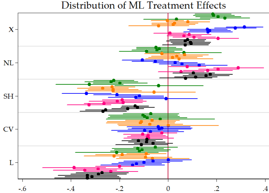
Figure 32: This figure plots the distribution of \hat{\alpha}_F^{(h,v)} from equation (11) done by (h, v) subsets. That is, we are looking at the average partial effect on the pseudo-OOS R^2 from augmenting the model with ML features, keeping everything else fixed. X is making the switch from data-poor to data-rich. Finally, variables are GDP, CONS, INV, INC and PCE. Within a specific color block, the horizon increases from h = 1 to h = 8 as we are going down. SEs are HAC. These are the 95% confidence bands.
