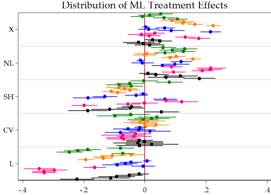
Figure 2: This figure plots the distribution of \hat{\alpha}_F^{(h,v)} from equation (11) done by (h, v) subsets. That is, we are looking at the average partial effect on the pseudo-OOS R^2 from augmenting the model with ML features, keeping everything else fixed. X is making the switch from data-poor to data-rich. Finally, variables are INDPRO , UNRATE , SPREAD , INF and HOUST. Within a specific color block, the horizon increases from h = 1 to h = 24 as we are going down. As an example, we clearly see that the partial effect of X on the R^2 of INF increases drastically with the forecasted horizon h . SEs are HAC. These are the 95% confidence bands.
