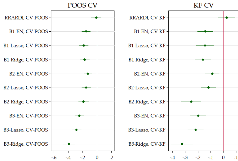
Figure 36: This compares models of section 3.2 averaged over all variables and horizons. The unit of the x-axis are improvements in OOS R^2 over the basis model. The base models are ARDIs specified with POOS-CV and KF-CV respectively. SEs are HAC. These are the 95% confidence bands.
