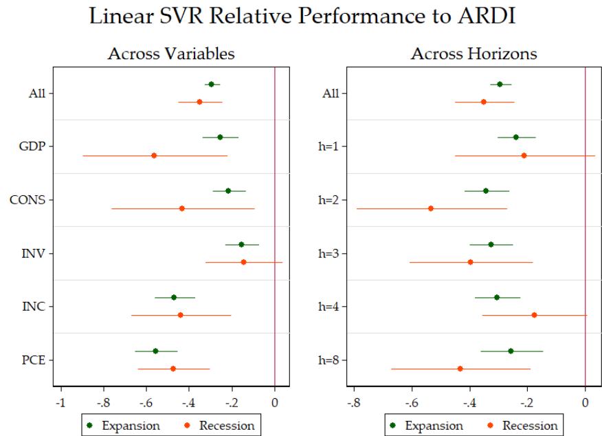
Figure 39: This graph display the marginal (un)improvements by variables and horizons to opt for the SVR in-sample loss function in both the data-poor and data-rich environments . The unit of the x-axis are improvements in OOS R^2 over the basis model. SEs are HAC. These are the 95% confidence bands.
