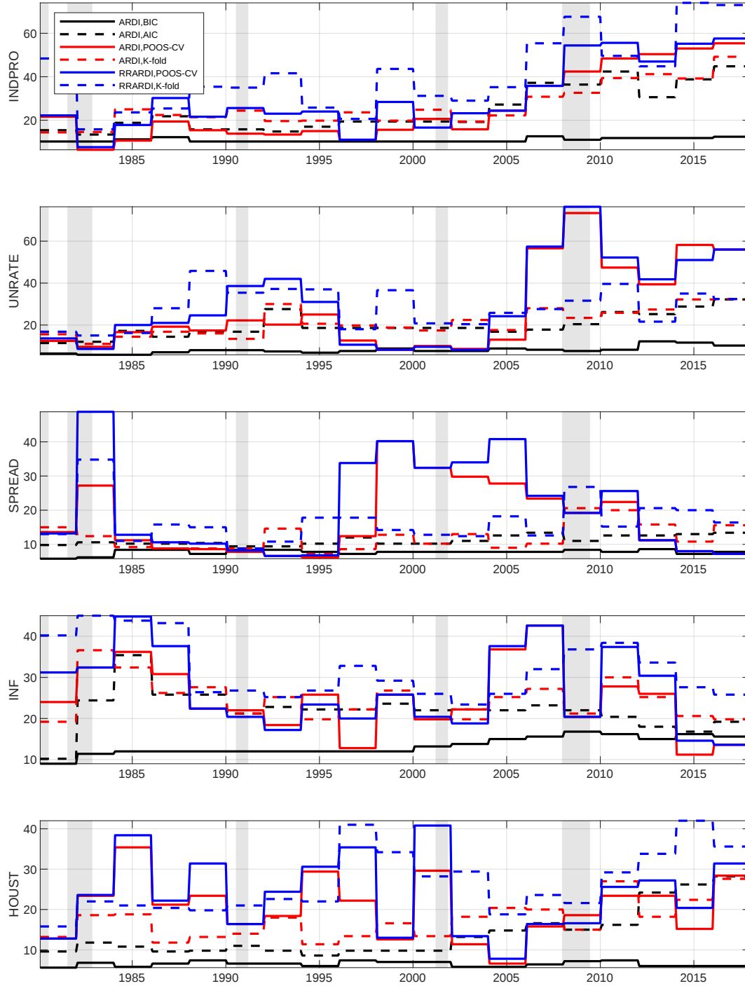
Figure 7: This figure shows the number of regressors in linear ARDI models. Results averaged across horizons.
