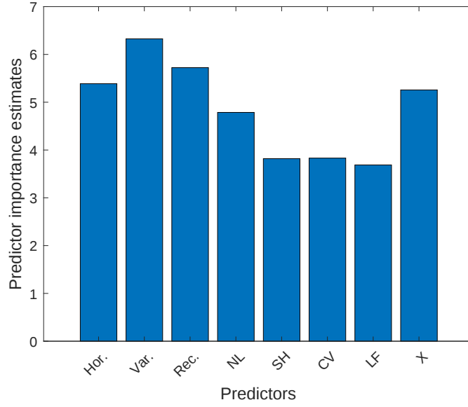
Figure 21: This figure presents predictive importance estimates. Random forest is trained to predict R^1_{t,h,v,m} defined in (11) and use out-of-bags observations to assess the performance of the model and compute features' importance. NL, SH, CV and LF stand for nonlinearity, shrinkage, cross-validation and loss function features respectively. A dummy for H_t^+ models, X , is included as well.
