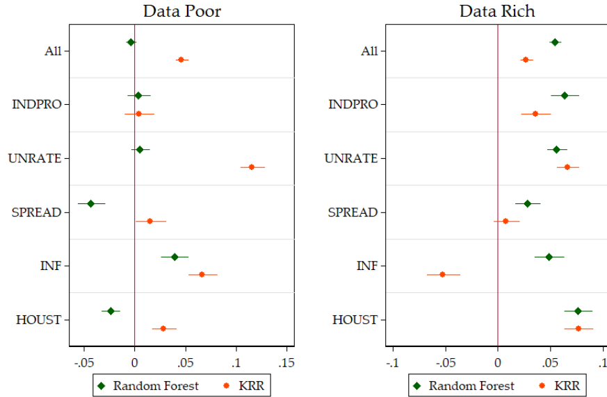
Figure 24: This compares the two NL models averaged over all horizons. The unit of the x-axis are improvements in OOS R^1 over the basis model. SEs are HAC. These are the 95% confidence bands.
