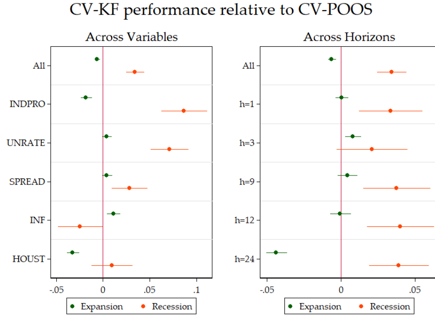
Figure 28: This compares the two CVs procedure averaged over all the models that use them. The unit of the x-axis are improvements in OOS R^1 over the basis model. SEs are HAC. These are the 95% confidence bands.
