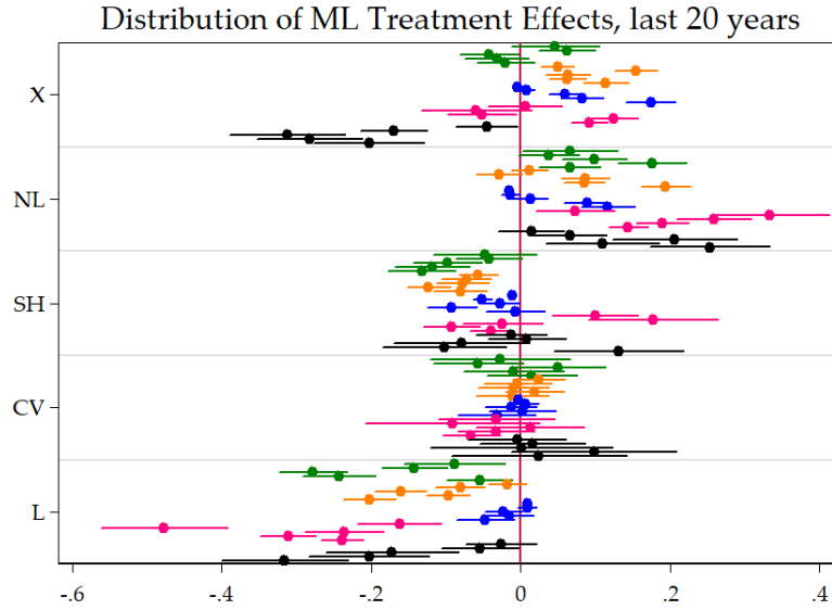
Figure 16: This figure plots the distribution of \hat{\alpha}_F^{(h,v)} from equation 11 done by (h, v) subsets. The subsample under consideration here are the last 20 years . The unit of the x-axis are improvements in OOS R^2 over the basis model. Variables are INDPRO , UNRATE , SPREAD , INF and HOUST . Within a specific color block, the horizon increases from h = 1 to h = 24 as we are going down. SEs are HAC. These are the 95% confidence bands.
