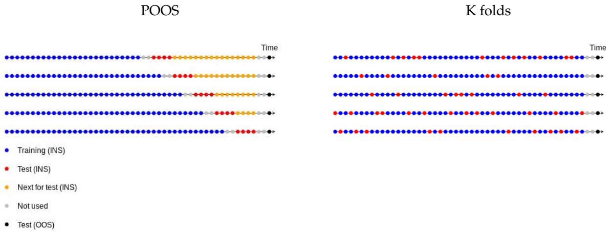
Figure 43: Illustration of cross-validation methods
