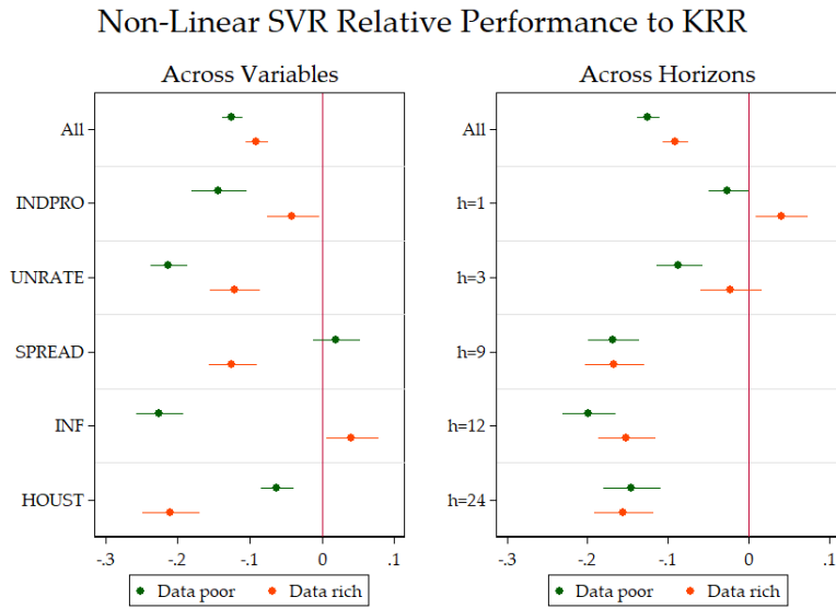
Figure 20: This graph display the marginal (un)improvements by variables and horizons to opt for the SVR in-sample loss function in comparing the data-poor and data-rich environments for nonlinear models. The unit of the x-axis are improvements in OOS R^2 over the basis model. SEs are HAC. These are the 95% confidence bands.
