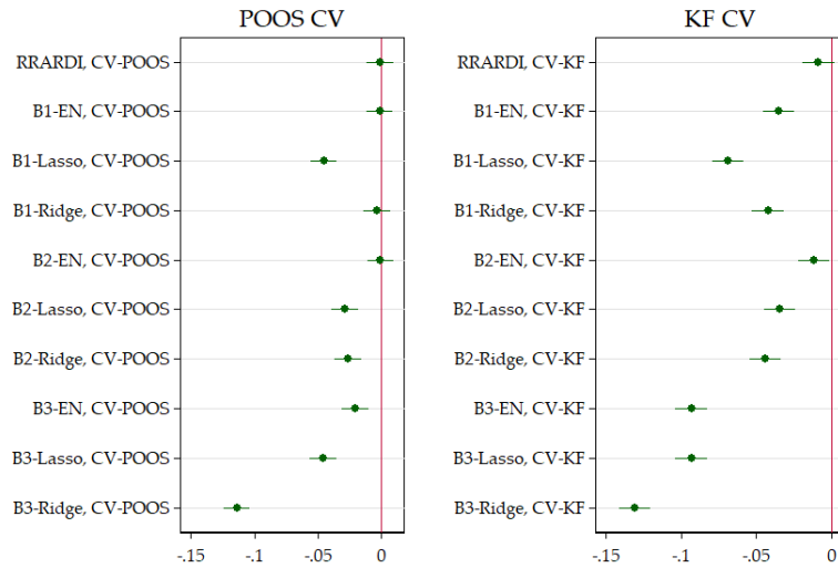
Figure 26: This compares models of section 3.2 averaged over all variables and horizons. The unit of the x-axis are improvements in OOS R^1 over the basis model. The base models are ARDIs specified with POOS-CV and KF-CV respectively. SEs are HAC. These are the 95% confidence bands.
