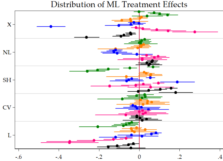
Figure 42: This figure plots the distribution of \hat{\alpha}_F^{(h,v)} from equation (11) done by (h, v) subsets. That is, we are looking at the average partial effect on the pseudo-OOS R^2 from augmenting the model with ML features, keeping everything else fixed. X is making the switch from data-poor to data-rich. Finally, variables are INDPRO , UNRATE , SPREAD , INF and HOUS. Within a specific color block, the horizon increases from h = 1 to h = 24 as we are going down. SEs are HAC. These are the 95% confidence bands.
