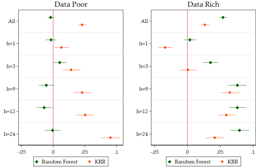
Figure 25: This compares the two NL models averaged over all variables. The unit of the x-axis are improvements in OOS R^1 over the basis model. SEs are HAC. These are the 95% confidence bands.
