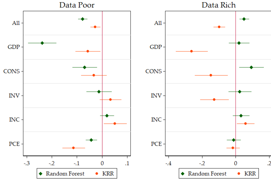
Figure 34: This compares the two NL models averaged over all horizons. The unit of the x-axis are improvements in OOS R^2 over the basis model. SEs are HAC. These are the 95% confidence bands.
