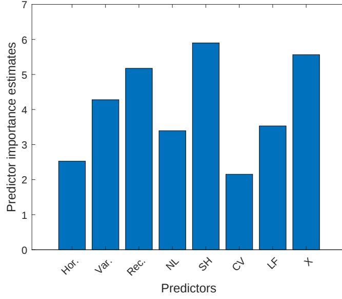
Figure 31: This figure presents predictive importance estimates. Random forest is trained to predict R_{t,h,v,m}^2 defined in (11) and use out-of-bags observations to assess the performance of the model and compute features' importance. NL, SH, CV and LF stand for nonlinearity, shrinkage, cross-validation and loss function features respectively. A dummy for H_t^+ models, X , is included as well.
