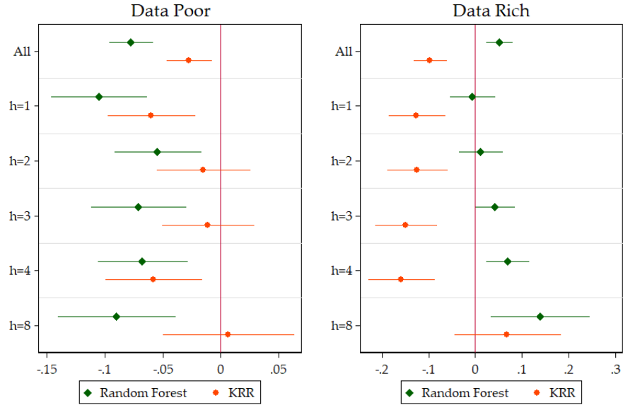
Figure 35: This compares the two NL models averaged over all variables. The unit of the x-axis are improvements in OOS R^2 over the basis model. SEs are HAC. These are the 95% confidence bands.
