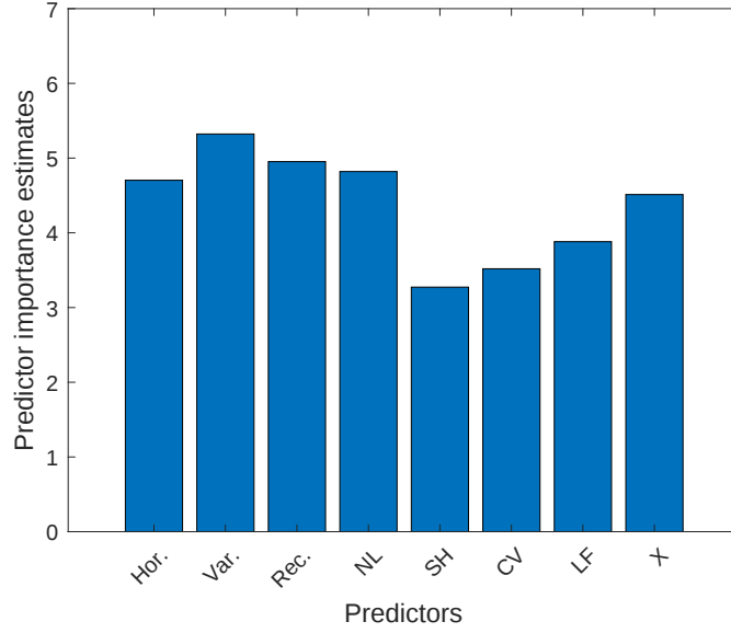
Figure 1: This figure presents predictive importance estimates, (Breiman, 2001). Random forest is trained to predict R_{t,h,v,m}^2 defined in (11) and use out-of-bags observations to assess the performance of the model and compute features' importance. NL, SH, CV and LF stand for nonlinearity, shrinkage, cross-validation and loss function features respectively. A dummy for H_t^+ models, X , is included as well.
