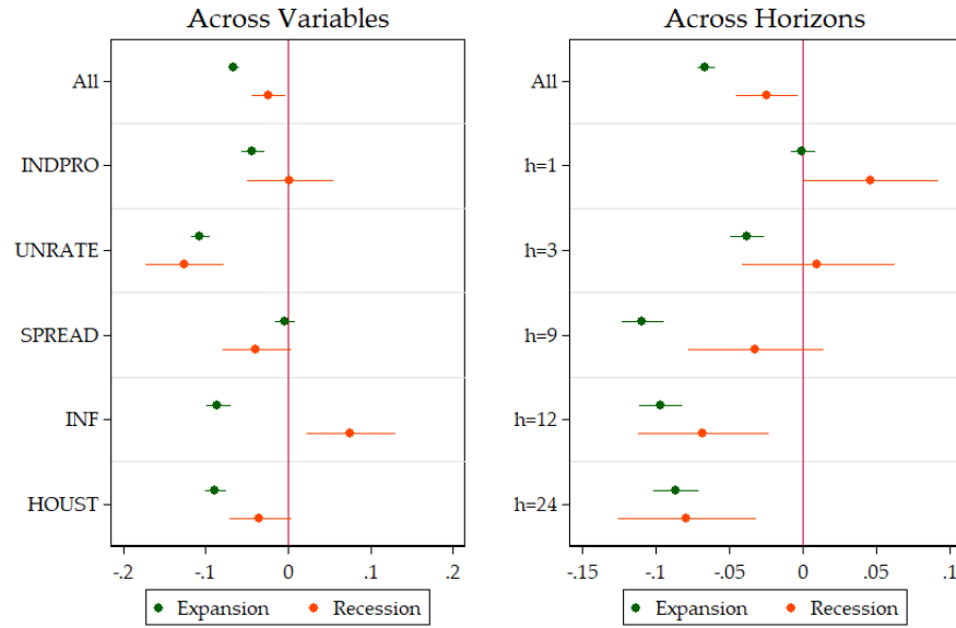
Figure 30: This graph display the marginal (un)improvements by variables and horizons to opt for the SVR in-sample loss function in both recession and expansion periods . The unit of the x-axis are improvements in OOS R^2 over the basis model. SEs are HAC. These are the 95% confidence bands.
