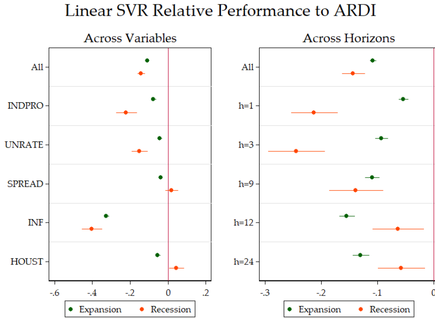
Figure 29: This graph display the marginal (un)improvements by variables and horizons to opt for the SVR in-sample loss function in both the data-poor and data-rich environments . The unit of the x-axis are improvements in OOS R^1 over the basis model. SEs are HAC. These are the 95% confidence bands.
