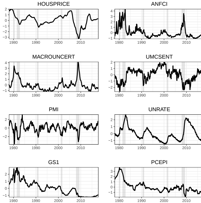
Figure 17: This figure plots time series of variables explaining the heterogeneity of NL treatment effects in section 6.
