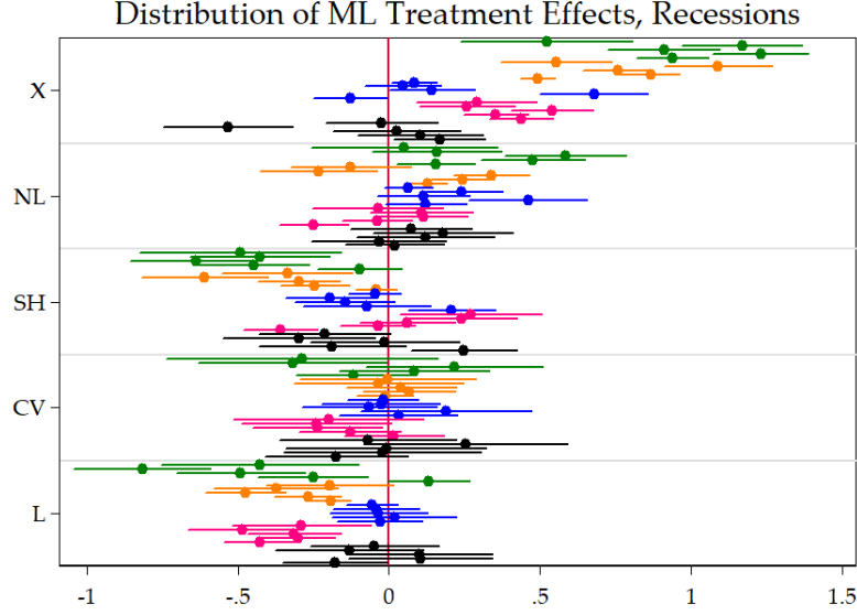
Figure 14: This figure plots the distribution of \hat{\alpha}_F^{(h,v)} from equation 11 done by (h, v) subsets. The subsample under consideration here are recessions . The unit of the x-axis are improvements in OOS R^2 over the basis model. Variables are INDPRO , UNRATE , SPREAD , INF and HOUST . Within a specific color block, the horizon increases from h = 1 to h = 24 as we are going down. SEs are HAC. These are the 95% confidence bands.
