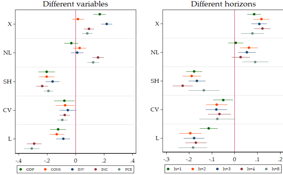
Figure 33: This figure plots the distribution of \hat{\alpha}_F^{(v)} and \hat{\alpha}_F^{(h)} from equation (11) done by h and v subsets. That is, we are looking at the average partial effect on the pseudo-OOS R^2 from augmenting the model with ML features, keeping everything else fixed. X is making the switch from data-poor to data-rich. However, in this graph, v -specific heterogeneity and h -specific heterogeneity have been integrated out in turns. SEs are HAC. These are the 95% confidence bands.
