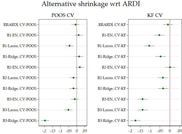
Figure 6: This figure compares models of section 3.2 averaged over all variables and horizons. The unit of the x-axis are improvements in OOS R^2 over the basis model. The base models are ARDIs specified with POOS-CV and KF-CV respectively. SEs are HAC. These are the 95% confidence bands.
