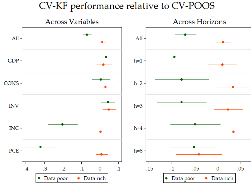
Figure 37: This compares the two CVs procedure averaged over all the models that use them. The unit of the x-axis are improvements in OOS R^2 over the basis model. SEs are HAC. These are the 95% confidence bands.
