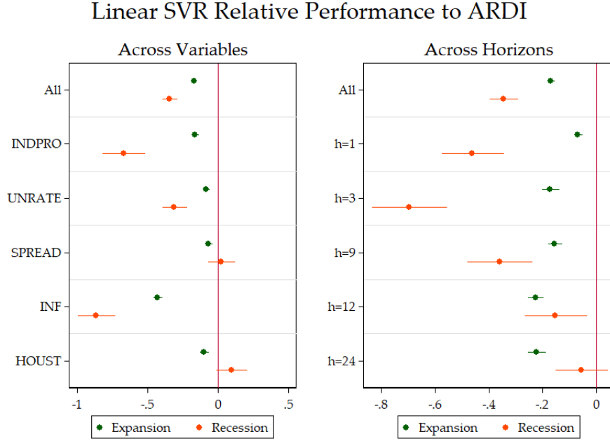
Figure 10: This graph displays the marginal (un)improvements by variables and horizons to opt for the SVR in-sample loss function in both recession and expansion periods. The unit of the x-axis are improvements in OOS R^2 over the basis model. SEs are HAC. These are the 95% confidence bands.
