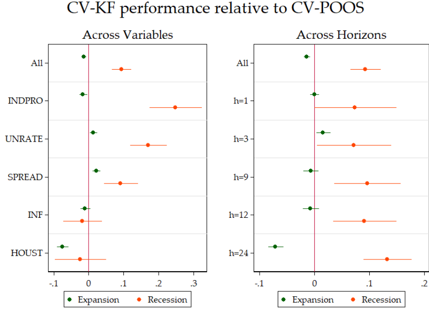
Figure 9: This figure compares the two CVs procedure averaged over all the models that use them. The unit of the x-axis are improvements in OOS R^2 over the basis model. SEs are HAC. These are the 95% confidence bands.
