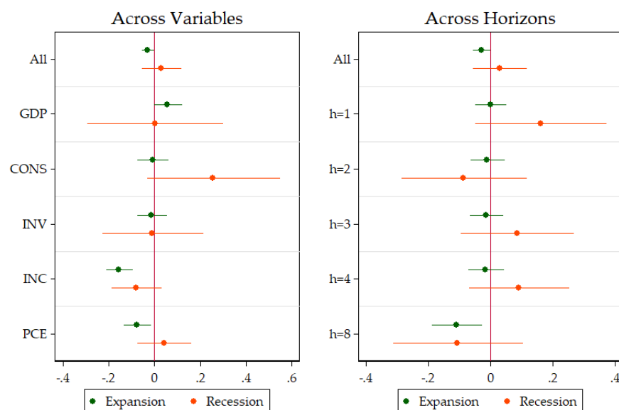
Figure 40: This graph display the marginal (un)improvements by variables and horizons to opt for the SVR in-sample loss function in both recession and expansion periods . The unit of the x-axis are improvements in OOS R^2 over the basis model. SEs are HAC. These are the 95% confidence bands.
