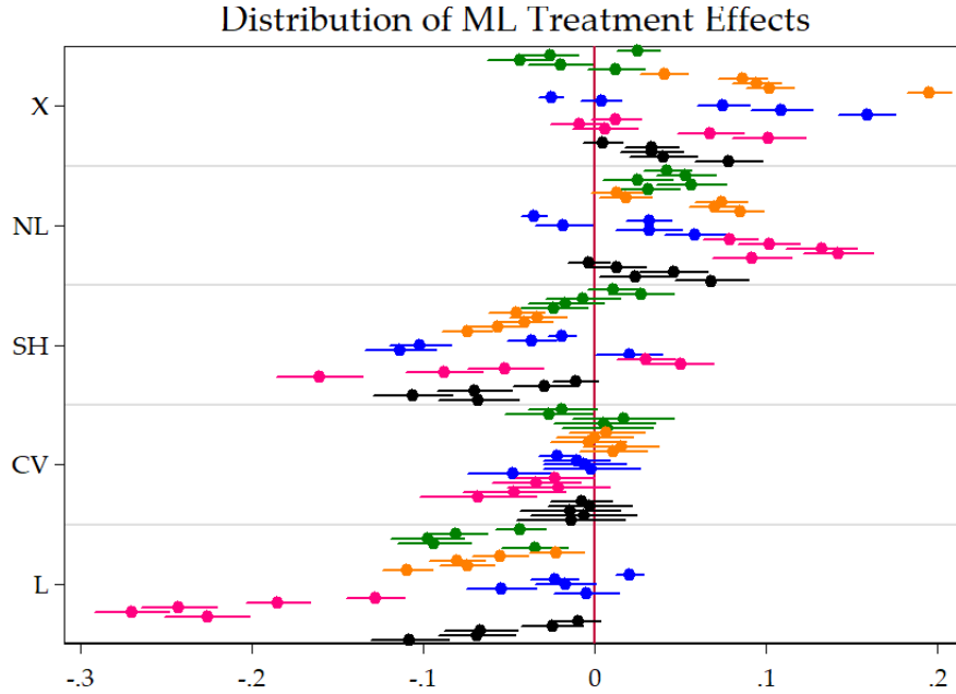
Figure 22: This figure plots the distribution of \hat{\alpha}_F^{(h,v)} from equation (11) done by (h, v) subsets. That is, we are looking at the average partial effect on the pseudo-OOS R^1 from augmenting the model with ML features, keeping everything else fixed. X is making the switch from data-poor to data-rich. Finally, variables are INDPRO , UNRATE , SPREAD , INF and HOUST. Within a specific color block, the horizon increases from h = 1 to h = 24 as we are going down. As an example, we clearly see that the partial effect of X on the R^1 of INF increases drastically with the forecasted horizon h . SEs are HAC. These are the 95% confidence bands.
