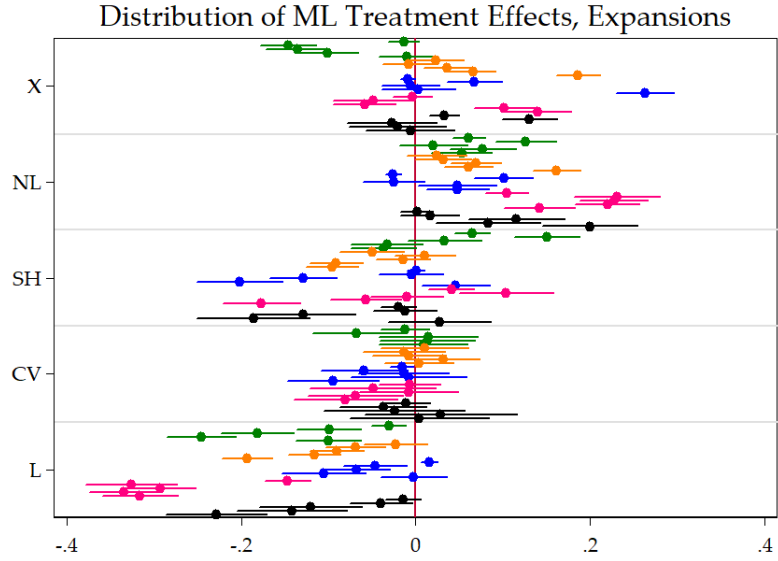
Figure 15: This figure plots the distribution of \hat{\alpha}_F^{(h,v)} from equation 11 done by (h, v) subsets. The subsample under consideration here are expansions . The unit of the x-axis are improvements in OOS R^2 over the basis model. Variables are INDPRO , UNRATE , SPREAD , INF and HOUST . Within a specific color block, the horizon increases from h = 1 to h = 24 as we are going down. SEs are HAC. These are the 95% confidence bands.
