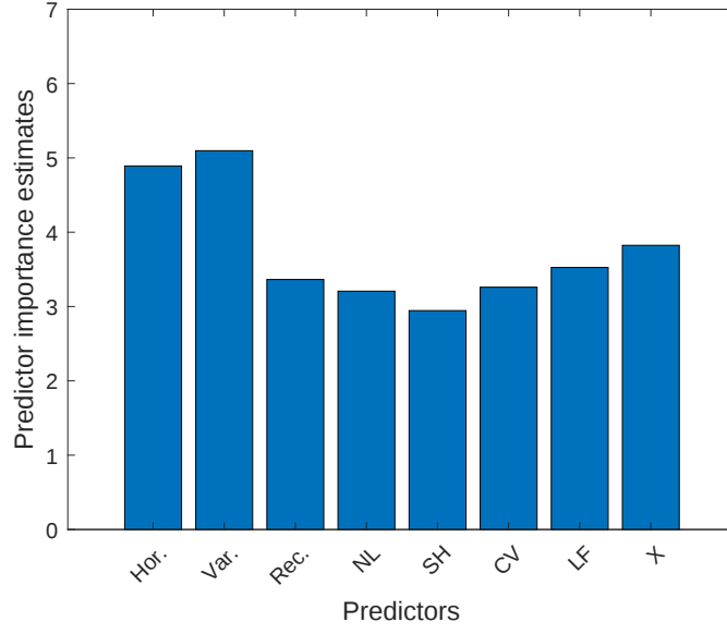
Figure 41: This figure presents predictive importance estimates. Random forest is trained to predict R^2_{t,h,v,m} defined in (11) and use out-of-bags observations to assess the performance of the model and compute features' importance. NL, SH, CV and LF stand for nonlinearity, shrinkage, cross-validation and loss function features respectively. A dummy for H_t^+ models, X , is included as well.
