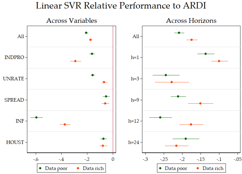
Figure 19: This graph display the marginal (un)improvements by variables and horizons to opt for the SVR in-sample loss function in comparing the data-poor and data-rich environments for linear models. The unit of the x-axis are improvements in OOS R^2 over the basis model. SEs are HAC. These are the 95% confidence bands.
