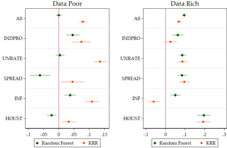
Figure 4: This figure compares the two NL models averaged over all horizons. The unit of the x-axis are improvements in OOS R^2 over the basis model. SEs are HAC. These are the 95% confidence bands.
