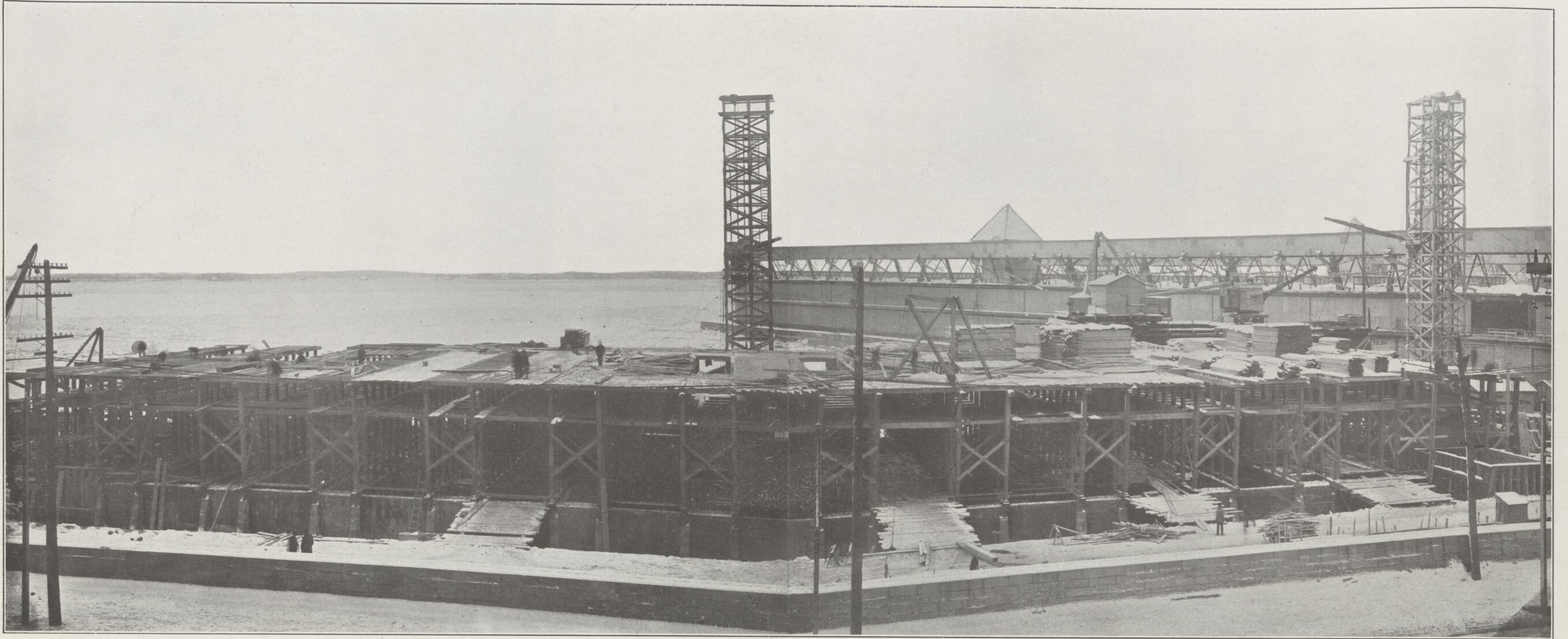
MONTREAL'S NEW HARBOR GRAIN ELEVATOR—This huge structure, now in course of erection, when completed, will be the largest grain-handling house in the world. It is being built by the Harbor Commissioners, and will be ready, it is hoped, for the reception of grain in September.
