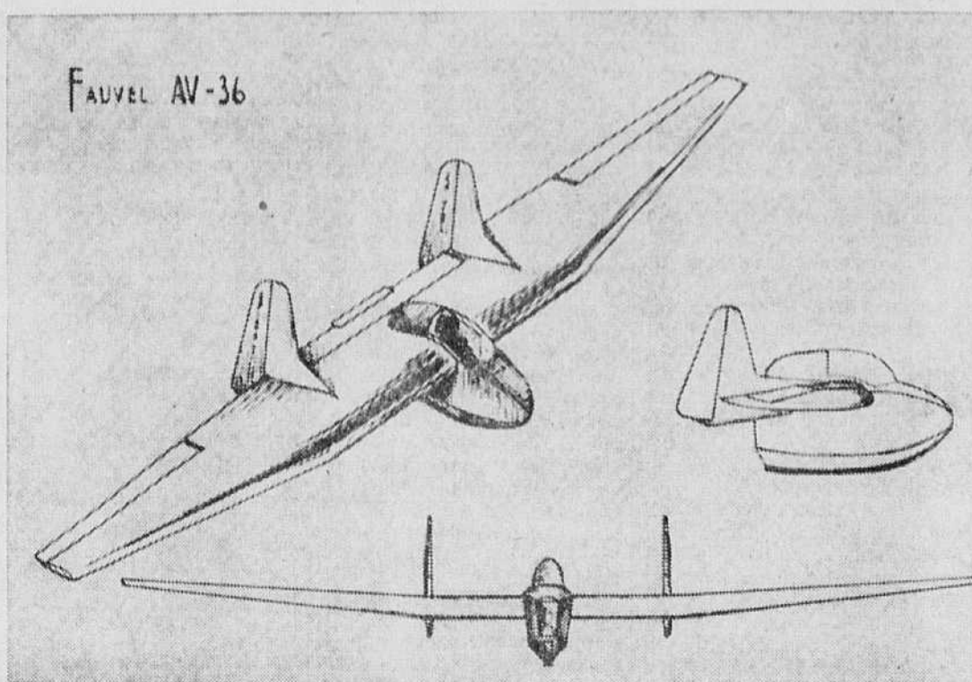
NEW GLIDER IN CONSTRUCTION HERE — Shown above are designs for a new Fauvel AV-36 glider which is being built by Jacques Codere in Sherbrooke. There is only one other similar ship in operation in Canada but there are several under construction by various glider clubs in the country. Mr. Codere expects to have his glider ready for a try-out by next summer. It will probably take him a total of 2000 hours to complete the all-wood construction. The Fauvel will have a wing span of 40 feet. There will be no tail or body, and the total length will be about seven feet. The pilot will sit in the small cockpit built right into the wing. One of the unique features of the glider is that it is built as one complete wing instead of a body with a wing on each side. When finished it will weigh about 250 pounds.
